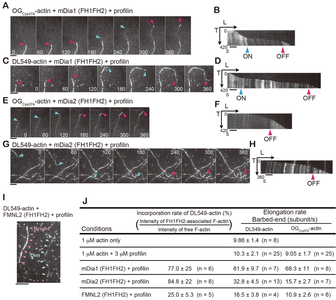
FIGURE 1: Incorporation of DL549-actin into formin-associated actin filaments in vitro. Actin assembly of 1 μM actin containing OG Cys374 -actin (10%) or DL549-actin (4%) in the presence of 3 μM profilin and 1 nM GST-mDia1ΔN3, 7.5 nM GST-mDia2 (FH1-FH2), or 7.5 nM GST-FMNL2 (FH1-FH2) on the glass coverslip coated with NEM-myosin II. (A, C, E, and G) Time-lapse images of actin growth of OG Cys374 -actin (A and E) or DL549-actin (C and G) with time in seconds indicated in images. Red arrows indicate the formin-free barbed ends growing at slow rates, and blue arrows indicate the barbed ends undergoing fast mDia1ΔN3-associated (A and C) or mDia2 (FH1-FH2)-associated (E and G) growth. The background spots in DL549-actin images represent nonspecifically bound single DL549-actin molecules on the glass surface. (B, D, F, and H) Kymographs show the length (x-axis) of OG Cys374 -actin filaments (B and F) or DL549-actin filaments (D and H) in (A, C, E, and G) vs. time (y-axis). Blue arrows indicate association (ON) of GST-mDia1ΔN3 or mDia2 (FH1FH2), and red arrows indicate dissociation (OFF) of formins. (I) Actin filaments assembled under the condition of 1 μM actin containing DL549-actin, 3 μM profilin, and 7.5 nM GST-FMNL2 (FH1-FH2) on a glass coverslip coated with NEM-myosin II. Pink arrows indicate a bright actin filament, and blue arrows indicate a dim filament. (A–I) Scale bars: 5 μm. (J) Summary of incorporation rates of DL549-actin to formin-associated filaments and elongation rates at barbed ends under indicated conditions. Rates are represented as mean ± SD.
