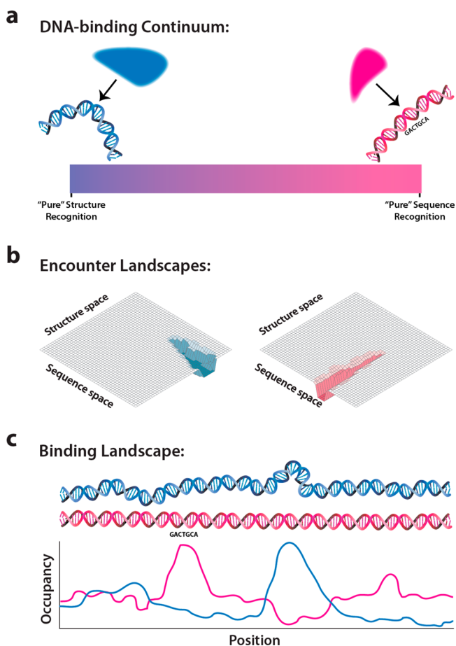
Figure 1. Principles contributing to DNA target recognition and binding by proteins. (a) Schematic illustration representing the DNA-binding continuum, the boundaries of which are defined by hypothetical examples of “structure interactor” or “sequence interactor”; real proteins are expected to fall somewhere in the continuum flanked by these two extremes. (b) Examples of hypothetical encounter landscapes: (left) protein whose binding behavior is dominated by DNA structure, and (right) protein whose target recognition properties are dominated by DNA sequence. (c) Binding landscape describes the stability of protein–DNA complexes along a defined DNA sequence.
