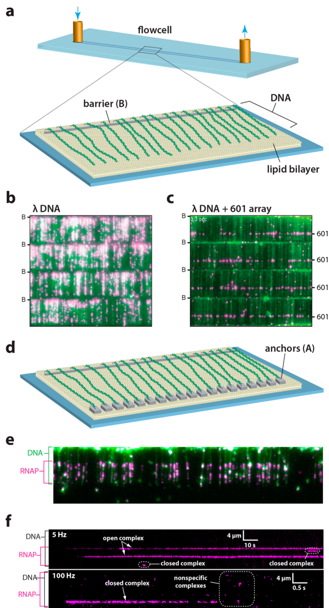
Figure 2. DNA curtains as a tool for studying protein–DNA interactions. (a) Schematic depiction a single-tethered DNA curtain in which one end of the DNA is anchored to a lipid bilayer and aligned along the leading edge of a nanofabricated barrier on the surface of the flow cell. 37g (b) Example of a 4-tiered DNA curtain bound by recombinant nucleosomes each of which is tagged with a fluorescent quantum dot. Lambda phage DNA is stained with YOYO1 and shown in green, the nucleosomes are in magenta, and the location of the nanofabricated barriers (B) are indicated. Adapted with permission from ref 37i. (c) Example of a DNA curtain made using a lambda phage DNA substrate containing a 13 \times array of the Widom 601 nucleosome positioning sequence (unpublished). (d) Schematic depiction a double-tethered DNA curtain in which one end of the DNA is anchored to a lipid bilayer and aligned along the leading edge of a nanofabricated barrier and the second end of the DNA is anchored to an antibody-coated pedestal. 37b (e) Wide-field TIRFM image showing quantum dot-tagged RNA polymerase (magenta) stably bound to the native promoters within the lambda phage genome. (f) Kymographs showing the association of RNA polymerase with an individual molecule of DNA (unlabeled) in real time. Adapted with permission from ref 37j.
