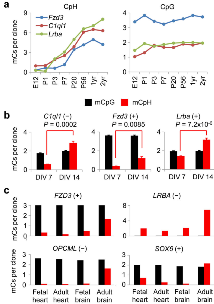
Figure 7. Establishment of CpH methylation during neuronal maturation
