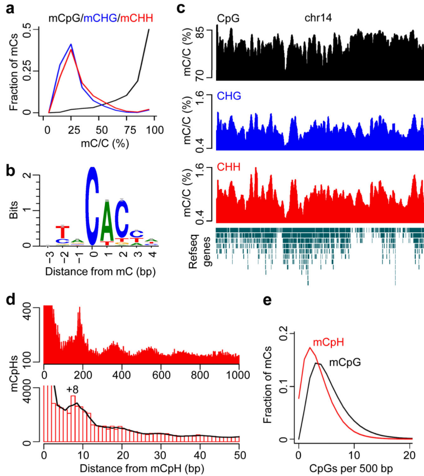
Figure 3. Genomic features of the neuronal CpH methylation (a) Distributions of methylation levels of mCpG (black), mCHG (blue) and mCHH (red) in the genome of adult mouse dentate granule neurons. (b) Motif analysis of all mCpHs, with mCs being in position 0. (c) A chromosome-wide view of three types of mCs on chromosome 14 (chr14). Methylation levels were moving-averaged by 100 kb windows. Refseq transcript annotation is shown at the bottom. (d) Spacing analysis of adjacent mCpHs. The cubic spline smoothing curve is shown. Please see comparison between adult dentate granule neurons and embryonic stem cells in Supplementary Fig. 5. (e) Relationship between mCpG/mCpH occurrence and their local CpG densities.
