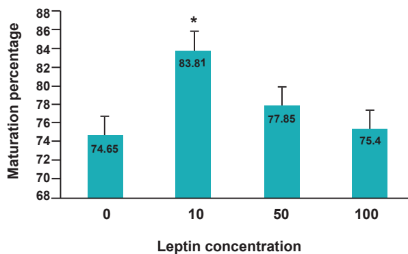
Fig 4: Effect of different leptin concentrations on oocyte maturation. There is a significant difference ( p < 0.05 ).
