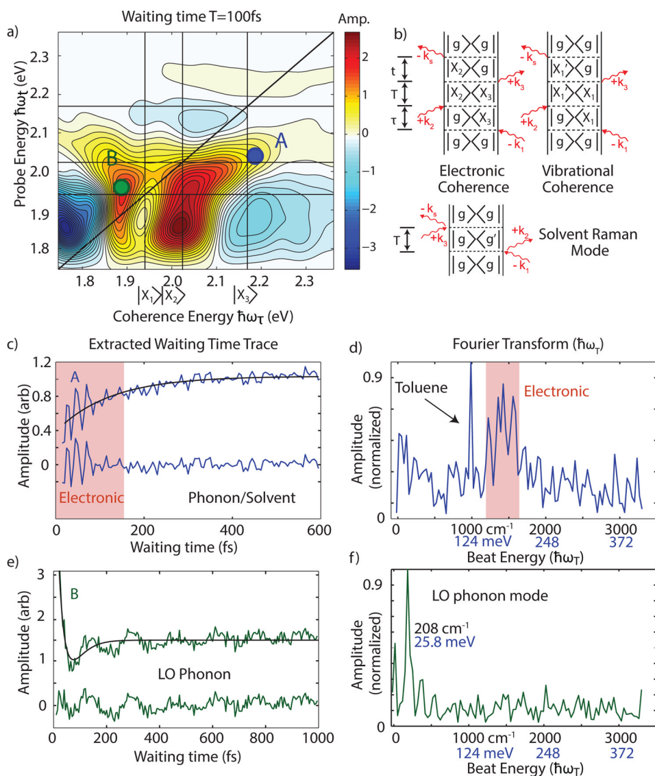
Figure 2. a) Two dimensional spectrum, with A representing the 1P/1S crosspeak, and B highlighting the band-edge feature. b) Feynman diagrams representing stimulated emission coherent oscillatory (rephasing \tau > 0 ) contributions to the signal, and coherent solvent response. The arrows represent electric field interactions, which interact with the density matrix of the ensemble. Coherences are off-diagonal elements of the density matrix, which during waiting time create oscillatory signals in 2D spectra. c) We plot the raw signal from A and the residual upon subtraction of a two fit exponentials representing population dynamics during waiting time. This shows large amplitude early time coherent response, followed by smaller amplitude oscillatory signals. d) A Fourier transform of the residual signal showing a broad peak centered at 1500 \text{ cm}^{-1} , assigned in this work to electronic coherence and a narrow peak near 1000 \text{ cm}^{-1} which we assign to the dominant Raman active mode in toluene. We attribute the apparent structure underneath the electronic coherence to additional solvent modes or to experimental noise. e) and f) show the same analysis as c) and d) for the band edge feature B , which oscillates with the longitudinal optical phonon mode.
