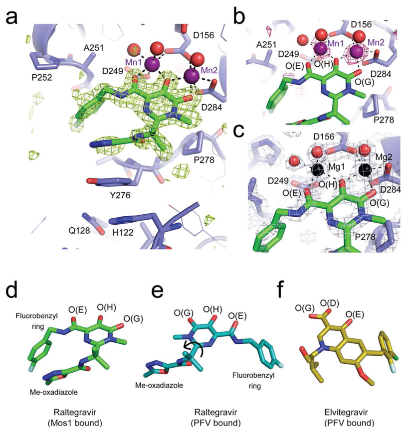
Figure 3. X-ray crystal structures of Raltegravir bound to the Mos1 transposase catalytic domain. (a) Active site of Mos1 transposase (blue) with Raltegravir (green sticks) bound to \text{Mn}^{2+} ions (purple spheres). The omit map of electron density (green mesh) is contoured at 3\sigma . Water molecules coordinated to the metal ions are displayed as red spheres. (b) Octahedral coordination of manganese ions in the active site, with anomalous difference electron density map contoured at 2.5\sigma (pink mesh). (c) Active site of the magnesium ion bound structure, with magnesium ions shown as black spheres. Conformations of Raltegravir bound to (d) Mos1 transposase catalytic domain and (e) the PFV intasome (PDB ID: 3OYA). Rotation about the CBC–CBF bond (indicated by a black arrow) would interconvert these two conformations. (f) Conformation of Elvitegravir bound to the PFV intasome (PDB ID: 3LSU).
