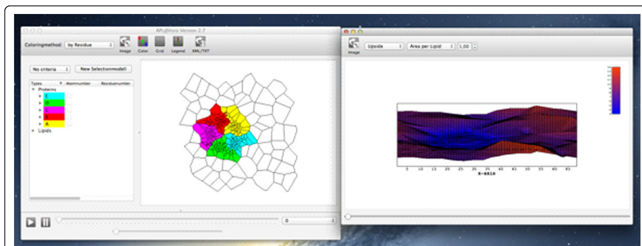
Figure 1 Pentamer of Vpu from HIV-1 in a POPC Bilayer. The Voronoi cells for the monomers are colored, the cells for the lipids are left in white.
