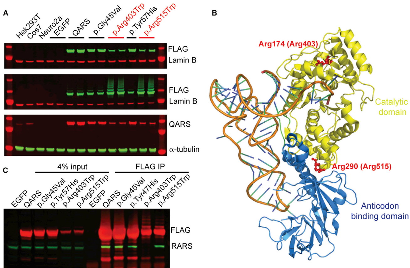
Figure 4. Effects of Individual Variants on QARS Solubility and Protein-Protein Interaction
