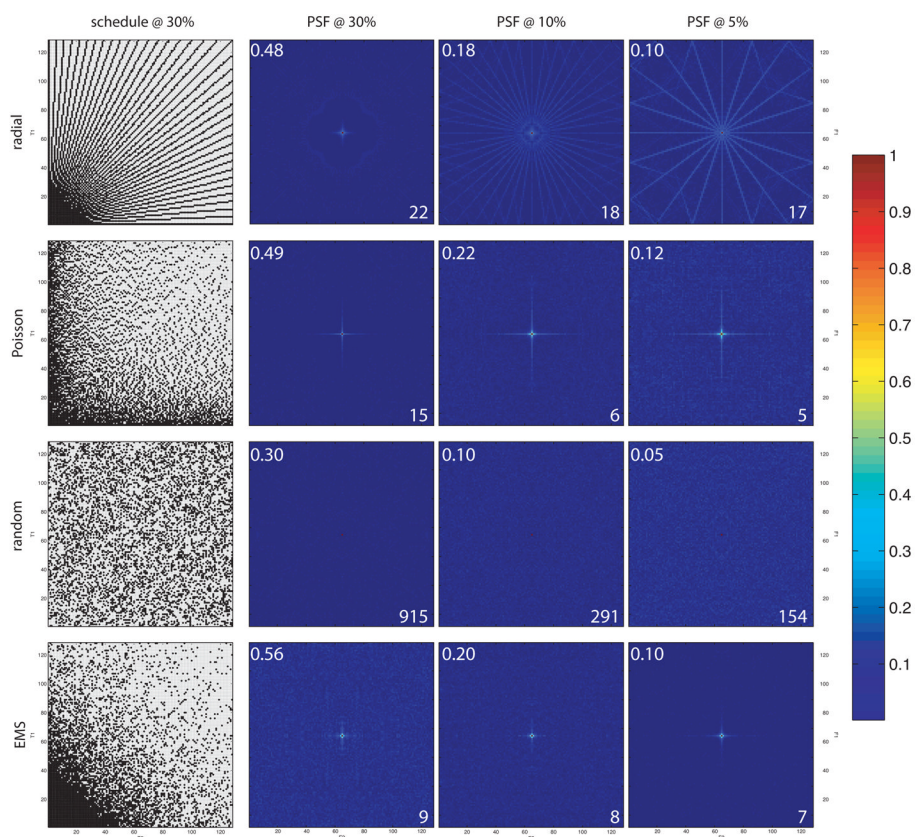
Figure 3. Examples of NUS schemes and PSFs
