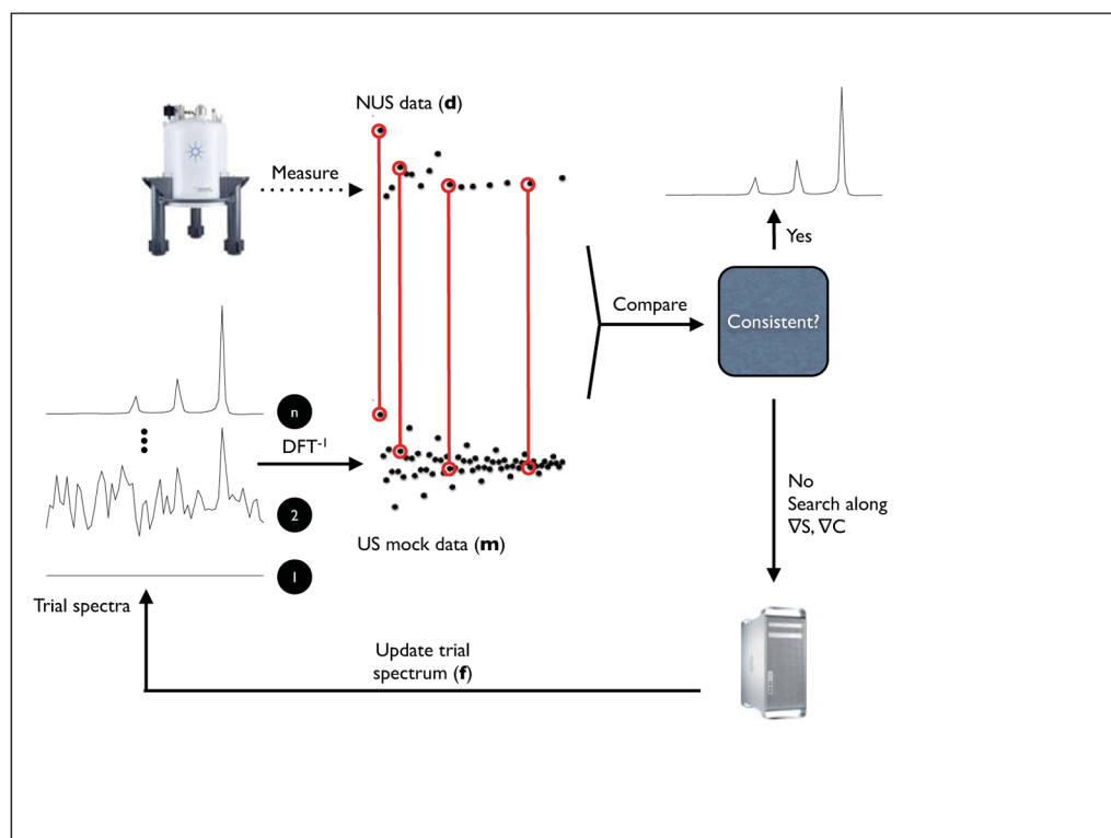
Figure 1. Schematic diagram for MaxEnt
