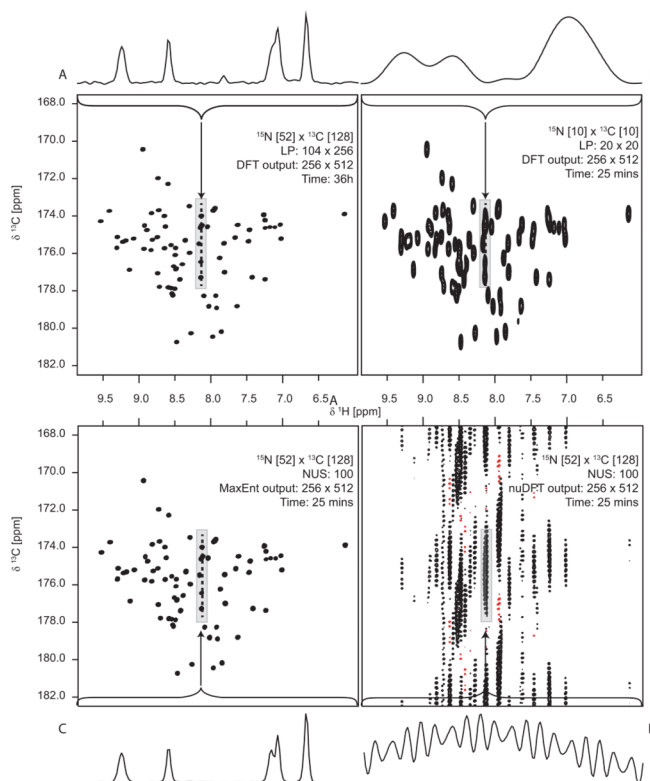
Figure 5. 3D HNCO spectra for Ubiquitin at 14.1 T (600 MHz for ^1\text{H} )
