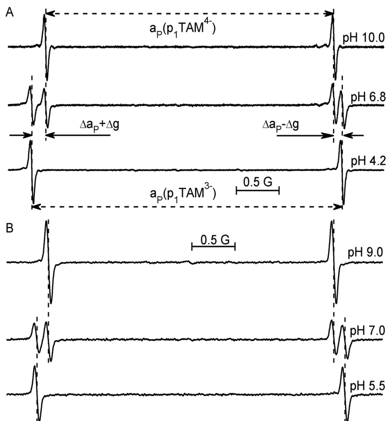
Figure 1. X-band (A) and L-band (B) EPR spectra of 0.1 mM (A) or 0.2 mM (B) solutions of p 1 TAM-D probe in 1 mM Na-phosphate buffer, 150 mM NaCl, measured at various pH values under nitrogen atmosphere and temperature of 37 °C.
