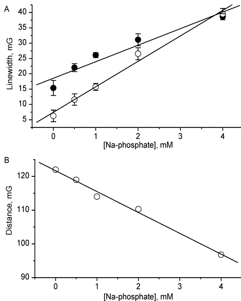
Figure 6. (A) Dependencies of the Lorentz linewidths of p 1 TAM 3- (●) and p 1 TAM 4- (○) components of p 1 TAM-D probe on phosphate buffer concentration. Solid lines represent the best linear fits with the slopes of (5.4 \pm 0.8) mG/mM and (8.3 \pm 0.5) mG/mM for p 1 TAM 3- and p 1 TAM 4- forms, correspondingly. (B) Dependence of distance between p 1 TAM 3- and p 1 TAM 4- components of p 1 TAM-D probe on phosphate buffer concentration. The solid line is the best linear fit with the slope of (6.2 \pm 0.3) mG/mM.
