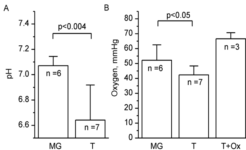
Figure 8. pH (A) and oxygen (B) values measured in mammary gland (MG) and tumor (T) tissues of the PyMT mice. Tumor tissue oxygenation was measured for air- and oxygen-breathing (T +Ox) animals. Average tumor size ( 0.9 \pm 0.4 cm 3 ). Error bars represent SD values.
