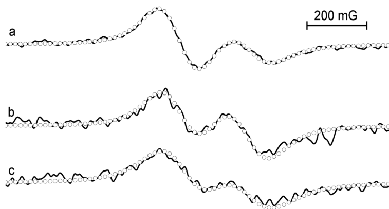
Figure 7. L-band EPR spectra of high-field component of p 1 TAM-D probe injected into the mammary gland (a) and tumor of the mouse breathing room air (b) or oxygen (c). Circles indicate simulated spectra yielding the p O 2 values 54 mmHg (a), 37 mmHg (b), and 66 mmHg (c), and pH values of 7.14 (a), 6.87 (b), and 6.84 (c). See Figure SI7 for the exemplified extraction of pH and p O 2 values by fitting experimental EPR spectra.
