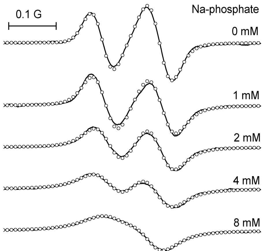
Figure 5. High-field component of the L-band EPR spectra of 200 \mu\text{M} p 1 TAM-D solution in Na-phosphate buffer, 150 mM NaCl, pH 6.8, measured at different buffer concentrations indicated near the spectra under anoxic conditions and temperature 37 °C. Symbols (○) represent the calculated spectra.
