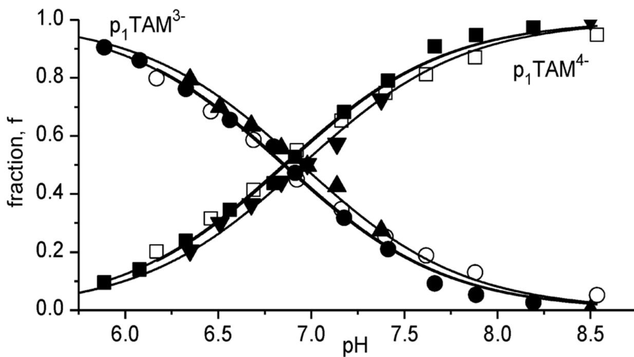
Figure 2. The pH dependencies of fraction of the ionization states of p_1TAM probes calculated from the corresponding X-band and L-band EPR spectra. The closed and open symbols denote the data obtained for deuterated and nondeuterated compounds, correspondingly; L-band data are shown by triangle symbols. Solid lines represent the best fits using standard titration equation yielding dissociation constant, pK_{a2} = 6.90 \pm 0.05 , for the second dissociation of phosphonic acid group of the probes.
