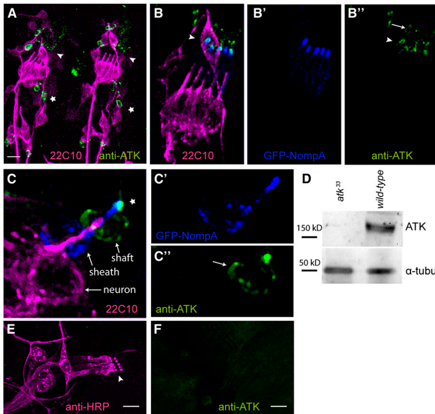
Figure 3 ATK localizes to the distal region of the dendritic cap in late embryonic mechanosensory organs. (A) Stage 16 embryonic hemisegments immunostained with the neuronal marker mAb22C10 (magenta) and with anti-ATK (green). ATK localizes apically to the sensory cilia in ch (arrowhead) and es (star) organs. (B and C) Detailed view of embryonic mechanosensory organs additionally showing GFP-NOMPA (blue) in the dendritic cap. Single channel images are shown for GFP-NOMPA (B' and C') and anti-ATK (B'' and C''). In lch5 (B) and es (C) organs, ATK localizes to the distal region of the dendritic cap (arrowhead in B, star in C), where it partially overlaps with GFP-NOMPA. The cytoplasm of cap and shaft cells are also stained (arrows). (D) Western blot with anti-ATK antibody. (E and F) ATK protein is not present in larval mechanosensory organs. Second instar larval lch5 organ stained with anti-HRP (E) shows no detectable anti-ATK staining. (F) Bars, 10 \mu m.
