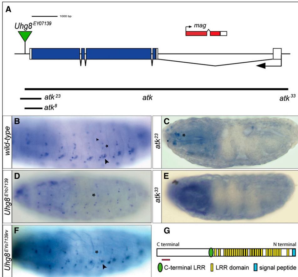
Figure 2 Generation of atk mutant alleles and anti-ATK antibody. (A) Schematic of atk locus. Shown are the location of the P{EPgy2} element Uhg8 EY07139 , extent of deletion in the alleles generated—hypomorphs atk 8 and atk 23 and null allele atk 33 —and location of the gene mag . (B–F) Stage 16 embryos hybridized with an atk anti-sense RNA probe. (B) Wild-type embryo showing hybridization in es organs (star) and ch organs (arrowhead). (C) atk 23 mutant embryos lack atk expression in mechanosensory organs, but expression persists in chemosensory organs (asterisk). (D) Embryos homozygous for Uhg8 EY07139 lose atk expression in ch organs (arrowhead in B and F) but keep it in es organs (star). (E) atk 33 homozygous embryos show no atk expression. (F) Uhg8 EY07139nv show normal atk expression. (G) Predicted ATK protein with 29 LRRs. Red line indicates the region against which anti-ATK antibody was raised.
