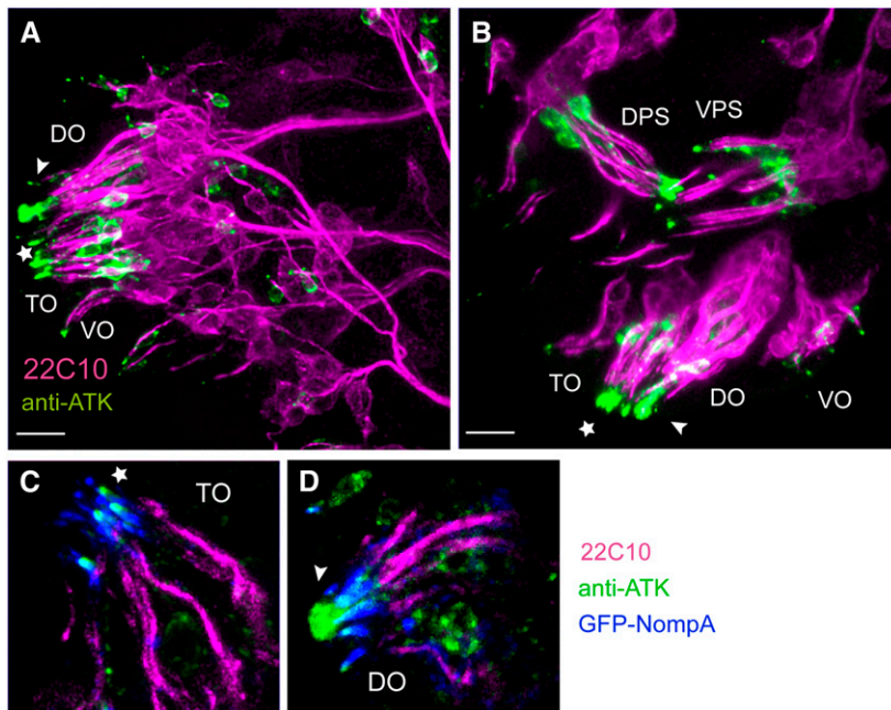
Figure 4 ATK localizes to a supporting ECM in late embryonic chemosensory organs. (A and B) Stage 16 embryonic chemosensory organs immunostained with the neuronal marker mAb22C10 (magenta) and anti-ATK (green). DO: dorsal organ; TO: terminal organ; VO: ventral organ; DPS: dorsal pharyngeal organ; VPS: ventral pharyngeal organ. In DO (arrowhead) and TO (star), ATK localizes to the tip of the chemosensory cilia. Cell bodies of atk -expressing cells are also stained. Bars, 10 \mu m. (C and D) Detailed view of TO (C) and DO (D) additionally showing GFP-NOMPA (blue). (C) In TO, ATK localizes at the tip of the GFP-NOMPA region (star), where gustatory neurons are exposed to the environment. (D) In DO, ATK forms a vacuole-like structure in the center of the cilia cluster (arrowhead).
