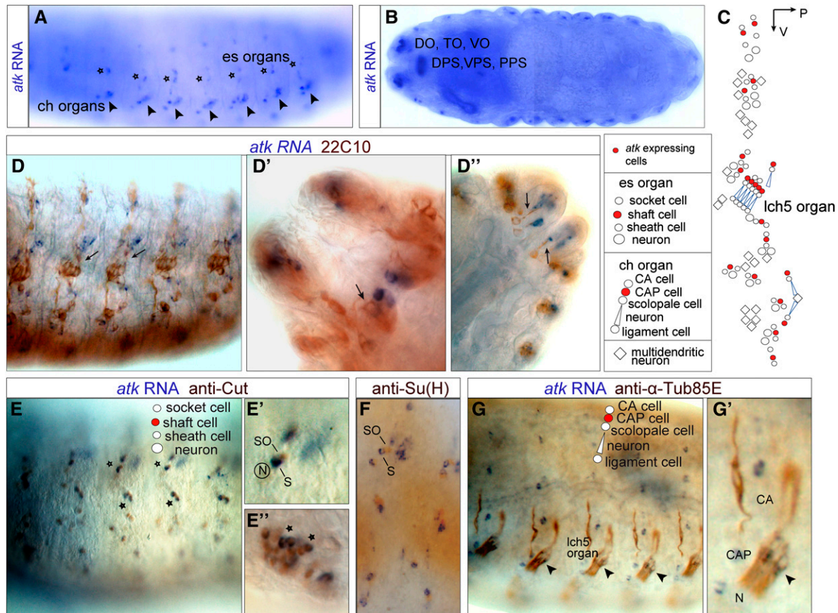
Figure 1 atk is expressed by an accessory cell in every ciliated sensory organ. (A and B) atk in situ hybridization in wild-type stage 16 embryos. (A) Lateral view showing atk in situ signal in a pattern consistent with expression in ch organs (arrowheads) and es organs (stars). (B) Horizontal view showing atk expression in chemosensory organs: dorsal organ (DO), terminal organ (TO), ventral organ (VO), dorsal, ventral and posterior pharyngeal organs (DPS, VPS, and PPS, respectively). (C) Schematic diagram of mechanosensory organs per hemisegment showing atk -expressing cells (red). (D–G) Embryos double-stained for atk in situ (blue signal) and different primary antibodies (brown signal). (D) atk is not expressed by ciliated neurons labeled by the neuronal marker mAb 22C10 (arrows, D–D’). (E and F) In es and chemosensory organs, atk is expressed by the shaft cell: it colocalizes with anti-Cut signal (stars, E–E’), which labels socket (SO) and shaft (S) cells, but does not colocalize with anti-Su(H), which labels the socket (F). (G) In ch organs, atk is expressed by the cap cell (CAP) based on atk -expressing cell position and colocalization with anti- \alpha -Tub85E (arrowheads, G and G’). CA: cap attachment cell; N: neuron.
