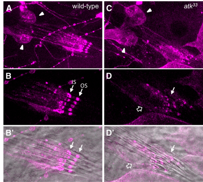
Figure 6 atk mutant larvae show abnormal lch5 organ morphology and altered anti-HRP signal in cilia. Third instar larval lch5 organs stained with anti-HRP (magenta) in control (A and B) and atk 33 mutants (C and D). (A and C) General view of neuronal cell bodies (arrowheads) and cilia. (B and D) High magnification of cilia showing anti-HRP signal, alone (B and D) or merged with a bright-field image (B' and D'). In control lch5 organs (B), cilia are parallel and aligned with anti-HRP signal concentrated in two bands corresponding to inner (IS) and outer (OS) segments (Ma and Jarman 2011). In atk mutants (D), alignment of cilia is lost (open arrow points to a cilium that is bent and separated from the others), and distribution of anti-HRP immunoreactivity is severely disrupted.
