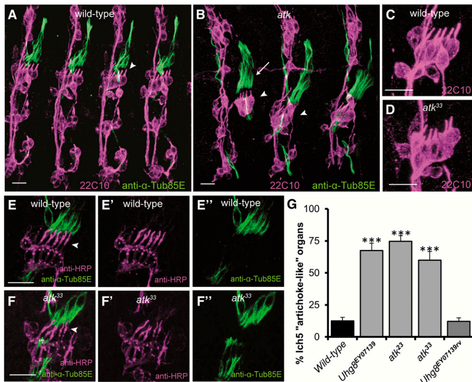
Figure 5 atk mutants show abnormal embryonic lch5 organ morphology. (A–D) Stage 16 embryonic hemisegments stained with neuronal marker mAb22C10 (magenta, labeling cell body and inner dendritic segment) and anti- \alpha -Tub85E (green), which labels all ch organ accessory cells except the scolopale cell. (A and C) In wild-type lch5 organs, sensory cilia are parallel and point in the same direction (arrowhead). Neuronal cell bodies are aligned in a row. (B and D) In atk 33 embryos, many lch5 organs show an artichoke-like phenotype with nonparallel dendrites and misaligned cell bodies (arrowheads in B). Cap cells also show defects (arrow in B). (E and F) Lch5 organs of stage 16 embryos, stained with anti-HRP (magenta, E' and F') that labels the entire cilium, and anti- \alpha -Tub85E (green, E'' and F''). The cilium tip contacts the dendritic cap in both wild-type (E, arrowhead) and atk 33 mutants (F, arrowhead). Bars, 10 \mu m. (G) Percentage of artichoke-like lch5 organs per hemisegment and genotype. Embryos were stained with mAb22C10 to label the sensory neurons and scored blind to genotype. Significant difference was established by the Kruskal–Wallis test followed by a nonparametric post-hoc test to compare each genotype with wild type. *** p < 0.001 .
