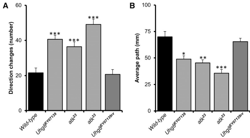
Figure 7 atk mutants show larval locomotion defects. Locomotion was scored for 100 sec by measuring the total number of direction changes (A) and the average path length (mm) (B). Means are represented. Error bars indicate SEM. Significant difference with respect to wild type was established by Bonferroni-corrected t -test. * P < 0.05; ** P < 0.01; *** P < 0.005.
