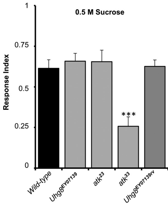
Figure 8 atk mutant larvae show a significantly reduced response to sucrose. Response index for election between 1% agarose and 1% agarose + 0.5 M sucrose. atk 33 null mutants show defects in chemosensation. atk 23 hypomorphs and Uhg8 EY07139 homozygous larvae, which keep atk expression in chemosensory organs, do not show defects. Therefore, ATK seems to be required for chemosensation, although an effect of additional genes deleted by the atk 33 deficiency cannot be ruled out. Error bars indicate SEM. Significant difference with respect to wild type was established by Bonferroni-corrected t -test. *** P < 0.001.
