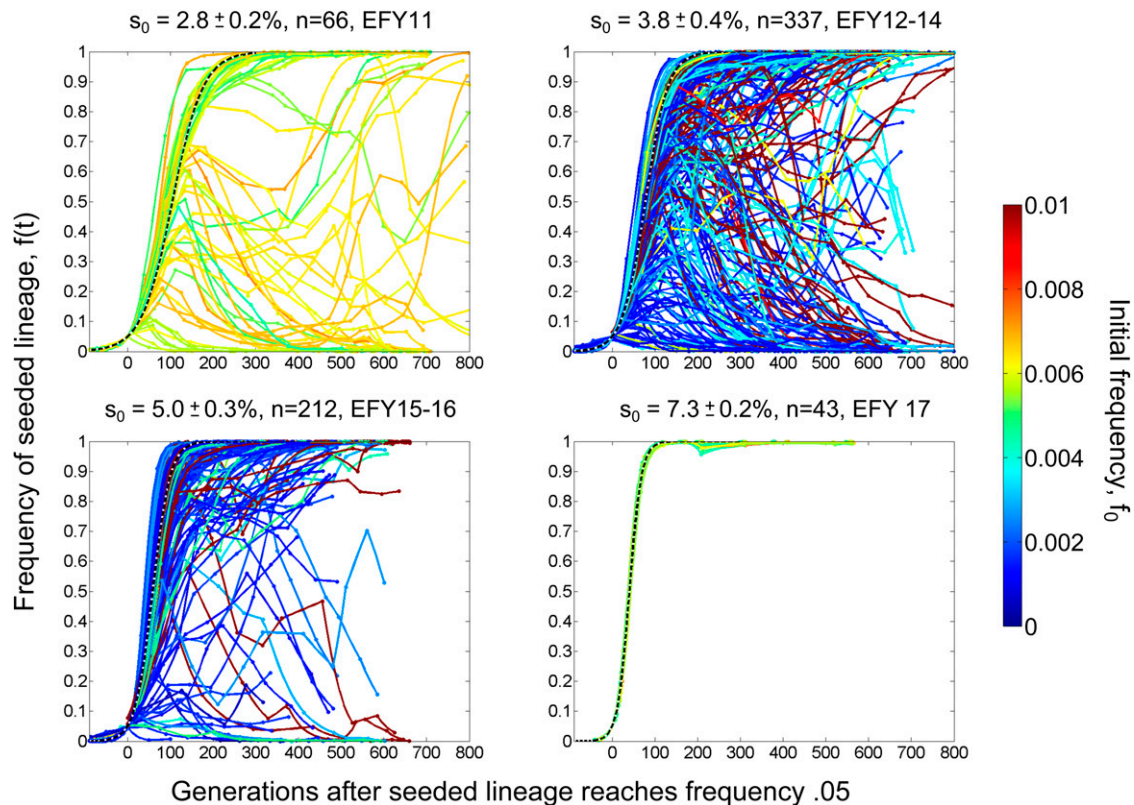
Figure 1 Trajectories of seeded lineages. Each line represents the frequency over time of a marked lineage with fitness advantage s_0 seeded into a replicate resident population. Colors correspond to the initial frequency f_0 of the seeded lineage according to the legend at right. Time is measured in generations, with t = 0 defined as the time at which each trajectory reached frequency 0.05. The dashed curves show the expected trajectories in the absence of new beneficial mutations ( i.e. , without clonal interference). (Note that the seeded lineages for s_0 \approx 4 and 5% consisted of multiple strains; see Materials and Methods .)
