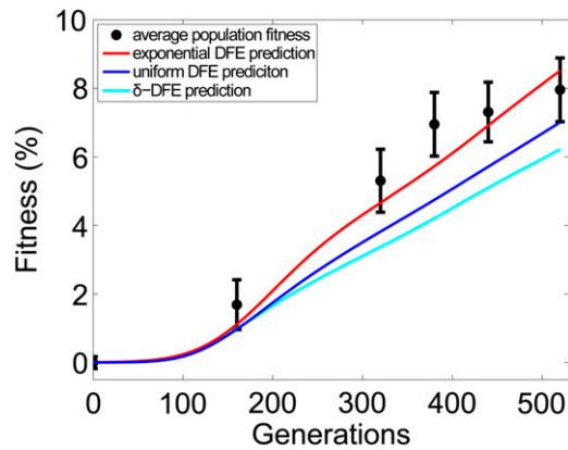
Figure 6 The rate of adaptation. The average fitness over time of 16 experimental control populations ( \pm 1 SEM) is shown in black. Solid curves are the predictions of these data given the most-likely exponential, uniform, and \delta -function DFEs. The fitnesses of individual populations are shown in Figure S4.
