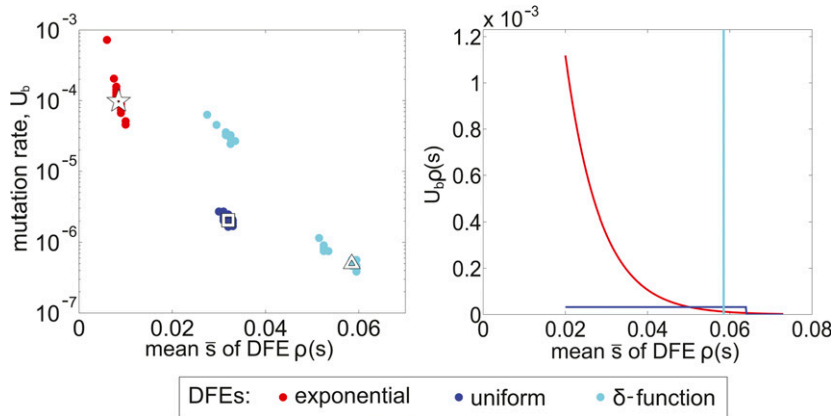
Figure 4 Inferred DFE parameters. Left: The most-likely parameters U_b and \bar{s} for DFEs \rho(s) given by exponential (star), uniform (square), and \delta -function (triangle) distributions. Shaded circles indicate 1% confidence ranges of these parameters as estimated by bootstrapping (see Appendix ). Right: The shapes of these distributions shown for s \geq 2\% given their most-likely parameters.
