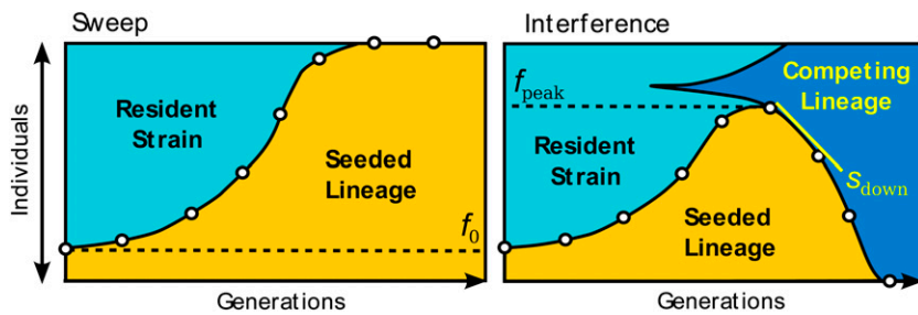
Figure 2 The fates of seeded lineages. We classified the trajectory of each seeded lineage according to whether it increased monotonically to fixation (a selective sweep, shown left) or peaked and subsequently declined in frequency (clonal interference, shown right). Each clonal interference event implies that the resident adapted fast enough to overtake the seeded lineage in fitness. These cases were further classified by the seeded lineage's peak frequency, f_{\text{peak}} , and relative fitness after this peak, s_{\text{down}} , as indicated in the right scheme.
