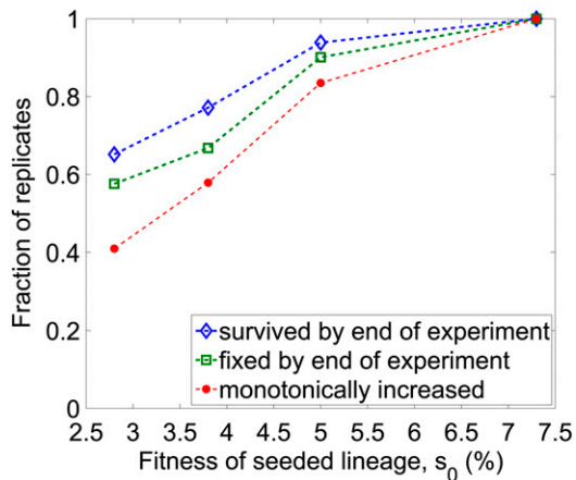
Figure 3 The fates of seeded lineages as a function of their fitness. We show the fraction of replicate populations in which the seeded lineage had the indicated fate.
