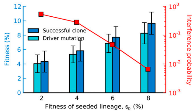
Figure 7 A screen for beneficial mutations. We simulated the evolutionary dynamics for a range of seeded lineages and then simulated picking a single clone at random from the resident population immediately after a clonal interference event. The bars indicate the average fitness of this clone and its largest effect mutation ( \pm 1 SD, scale at left). We also show the fraction of replicate populations in our simulations in which clonal interference occurs (scale at right). The simulations assumed the most-likely exponential DFE inferred in the study.
