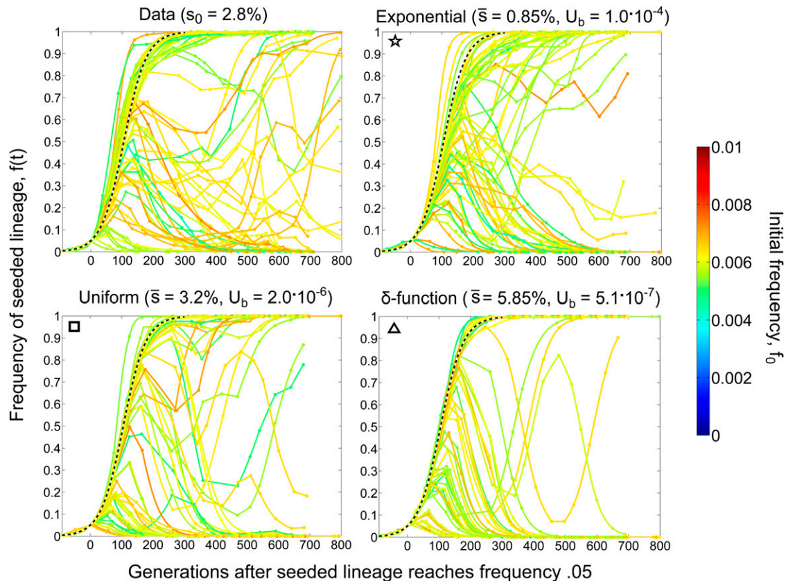
Figure 5 Lineage dynamics data and simulations for s_0 = 2.8\% . The trajectories of seeded lineages with initial fitness s_0 = 2.8\% are shown as observed in the experiment (top left) and as reproduced by simulations assuming the DFE parameters indicated above each part.
