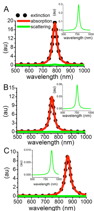
Figure 4. DDA extinction (black dots), absorption (red line), and scattering (green line, and shown in inset) spectra for the longitudinal mode of the different AuNRs in water. (A) The 38 × 10 nm AuNR has an absorbance:scattering ratio of 63.8. (B) The 25 × 7 nm AuNR has an absorbance:scattering ratio of 204. (C) The 18 × 4 nm AuNR has an absorbance:scattering ratio of 921.
