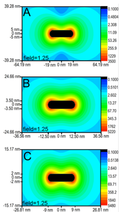
Figure 3. Field contour plots for the longitudinal mode of the different AuNRs, with particle dimensions indicated and the field decaying to 1.25 at the extremities of each plot. (A) The field maximum of the 38 \times 10 nm AuNR (calculated at 804 nm) is 3500. (B) The field maximum of the 25 \times 7 nm AuNR (calculated at 761 nm) is 5220. (C) The field maximum of the 18 \times 4 nm AuNR (calculated at 875 nm) is 5480.
