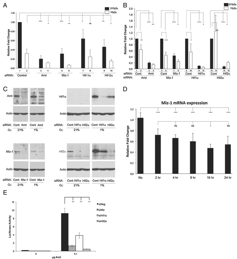
Figure 5 Inhibition of Miz-1, Arnt and Hifa expression reduces CDKN2B mRNA levels. A-C U2OS cells were transfected with siRNA (10 nM) against Arnt, Miz-1, Hif1α and Hif2α as indicated and cultured at normoxia (21% O 2 ) or hypoxia (1% O 2 ) for 6 hours. A ) qRT-PCR analyses of CDKN2B mRNA levels after administration of the different siRNAs are presented as relative fold changes compared to control siRNA at normoxia (column 1). B ) qRT-PCR analysis of mRNA expression of Arnt, Miz-1, Hif1α and Hif2α after siRNA treatment. The mRNA levels after administration of the different siRNAs are presented as relative fold changes compared to control siRNA at normoxia for each specific mRNA species. C ) Protein levels of Arnt (upper left panel), Miz-1 (lower left panel), Hif1α (upper right panel) and Hif2α (lower right panel) in response to siRNA treatment and hypoxia were determined by immunoblotting. Immunoblotting for beta-actin was included to control for protein loading. D ) U2OS cells were cultured at normoxia (21% O 2 ) or at hypoxia (1% O 2 ) for the time points indicated, and qRT-PCR analyses for Miz-1 mRNA expression were performed. The qRT-PCR values in A , B and D were normalized to the housekeeping gene HPRT-1, and are shown as average of two or three independent experiments performed in duplicates (n = 4 for A and B , n = 6 for D ). E ) U2OS cells were transfected with siRNA (10 nM) against Miz-1, Hif1α and Hif2α or a negative control siRNA together with the -35CDKN2B/luc reporter (300 ng) in the presence or absence of an Arnt expression vector (Arnt/Flag/pCMV, 100 ng) as indicated. The luciferase activity is presented as average ± stdev, n = 3. Statistical analyses: ( A-B and E ) Student's T -test, ( D ) ANOVA (Bonferroni); ***p ≤ 0.001, **P ≤ 0.01, *P ≤ 0.05, ns: non significant.
