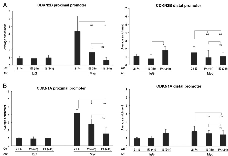
Figure 6 Hypoxia leads to release of Myc from the CDKN2B promoter. ChIP experiments were performed on extracts from U2OS cells using an antibody (Ab) against Myc or preimmune IgG as indicated. The cells were cultured at normoxia (21% O 2 ) or at hypoxia (1% O 2 ) for 4 or 24 hours before harvested. qPCR was performed with primers spanning the proximal (-168/-19) (A, left panel) or distal (-3874/-3744) (A, right panel) CDKN2B promoter sequences, and primers spanning either the proximal (+6/+106) (B, left panel) or distal (-2337/-2158) (B, right panel) CDKN1A promoter sequences. The results are given as average enrichment of the indicated promoter fragment +/- stdev, n = 6. Statistical analyses: ANOVA (Dunnett's T3), **P ≤ 0.01, *P ≤ 0.05, ns: not significant. For the IgG control experiments there were no statistically significant differences detected, apart from on the CDKN2B distal promoter, as indicated in the figure (A, right panel).
