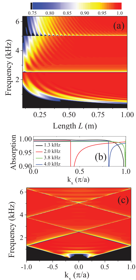
Figure 2 | Acoustic response of crystals made out of porous lamellas. (a), Absorption versus frequency and lamella length L for normal incident radiation where f = 30\% and W = 4 cm. (b,c), Simulated angular dependence of the structure in (a) with L = 0.5 m within the first Brillouin zone. We take illustrative examples corresponding to four frequency cuts in (c) and show the dependence of absorption with parallel momentum k_x .
