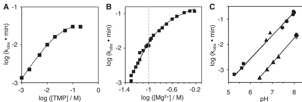
Figure 7. Dependence of reaction kinetics on reaction conditions, for the trans -splicing TPR1 ribozyme. (A) Dependence of the observed reaction rate on the concentration of TMP, with a free [\text{Mg}^{2+}] of 50 mM at pH 8.1. The maximal rate is reached at 100 mM [TMP]. The black line shows the fit of the Michaelis–Menten equation k_{\text{obs}} = (k_{\text{cat}} * [\text{TMP}] / (K_{\text{M}} + [\text{TMP}])) to data points from 1–100 mM [TMP], with k_{\text{cat}} = 0.039 \text{ min}^{-1} and K_{\text{M}} = 30 \text{ mM} . (B) Dependence of the observed reaction rate on the concentration of free magnesium ions. This is the excess of magnesium ions over the TMP concentration (here 100 mM), at pH 8.1. The dotted line separates reactions with [\text{Mg}^{2+}] / [\text{TMP}] < 1 (left) from reactions with [\text{Mg}^{2+}] / [\text{TMP}] > 1 (right). The fastest rate is obtained at 400 mM free [\text{Mg}^{2+}] . The half-maximal rate of 0.068 \text{ min}^{-1} was observed at 150 mM free [\text{Mg}^{2+}] . (C) Dependence of the observed reaction rate on the pH, at 100 mM [TMP] and 400 mM free [\text{Mg}^{2+}] (top line) and at 50 mM [TMP] and 50 mM free [\text{Mg}^{2+}] (bottom line). The slopes of the two lines were 0.92 (top line) and 0.99 (bottom line), respectively. The symbols denote the buffer systems MES/NaOH (squares), HEPES/NaOH (triangles) and Tris–HCl (circles). The data point in the lower data set at pH 8.1 is the average of seven independent experiments, with error bars denoting their standard deviation.
