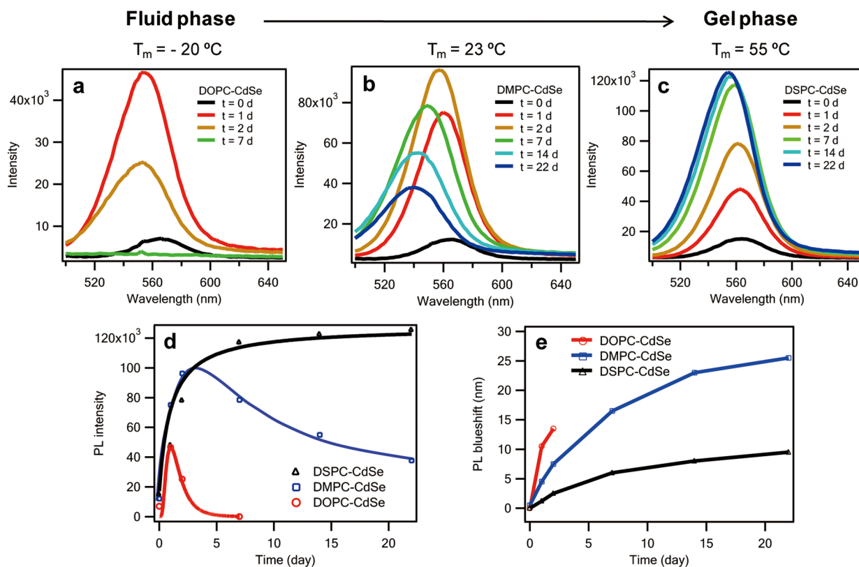
Figure 2. Membrane-dependent photostability of CdSe within L-QD assemblies. Time-dependent PL spectra of CdSe QDs in (a) DOPC, (b) DMPC, and (c) DSPC vesicles stored under ambient laboratory conditions. (d) Maxima PL intensity of L-QD vesicles as a function of time. (e) PL blue-shifts of L-QD vesicles as a function of time.
