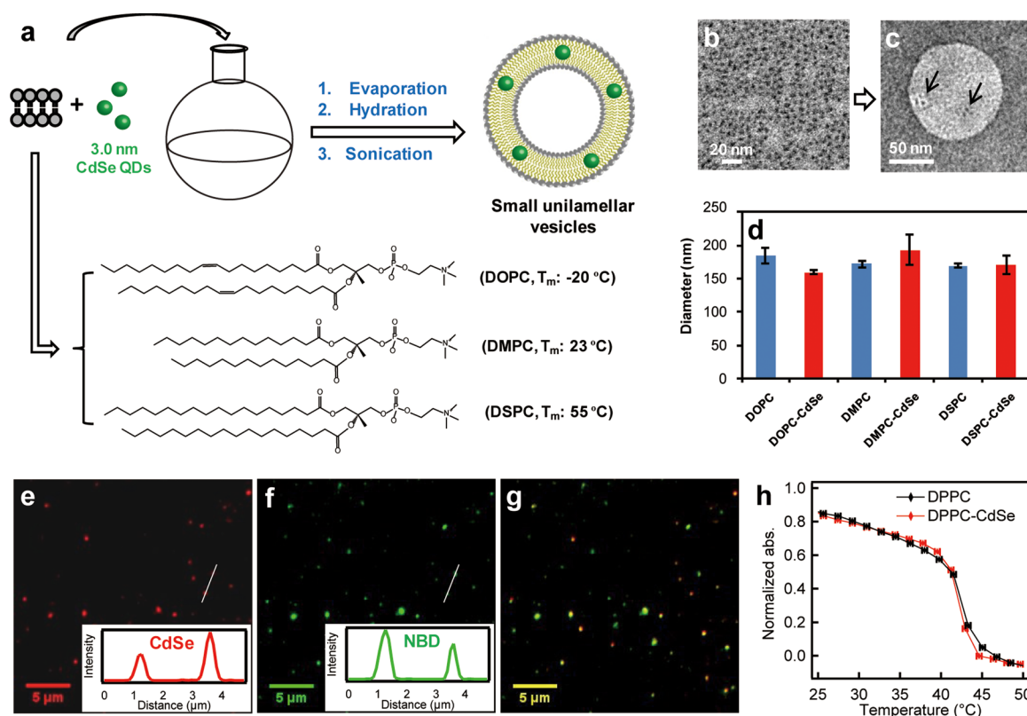
Figure 1. Formation and characterization of L-QD hybrid vesicles. (a) Formation of L-QD vesicles via solvent evaporation, hydration and probe sonication. (b and c) TEM image of CdSe QDs and negative stain TEM image of DSPC-CdSe vesicles. Arrows indicate the location of QDs. (d) Size of DOPC, DOPC-CdSe, DMPC, DMPC-CdSe, DSPC, and DSPC-CdSe vesicles obtained by DLS measurement. (e) and (f) are representative fluorescence images of CdSe QDs, and NBD-PC doped in DSPC vesicles. (g) is the merged image of (e) and (f), which shows colocalization of CdSe QDs and DSPC vesicles indicating the incorporation of QDs in the lipid membrane. Colocalization of CdSe QDs and DOPC vesicles is shown in Supporting Information Figure S3. (h) Thermal phase transition of DPPC and DPPC-CdSe vesicles obtained by plotting the intensity of the CH 2 stretch (2851 cm -1 ) versus temperature from temperature-dependent FT-IR spectra. 28
