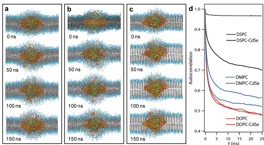
Figure 4. Atomistic MD simulation of L-QD assemblies. Representative snapshots of atomistic MD simulation of 2.6 nm CdSe nanocrystal (0–150 ns) in fluid phase DOPC (a), DMPC (b), and gel phase DSPC vesicles (c). Lipid tails and OA ligands are shown in gray and orange, respectively. Solvent is omitted for clarity. (d) Time correlation function of tail orientations for lipids perturbed by an embedded 2.6 nm CdSe QD (solid line) and lipids far from the QD (dotted line), averaged over the final 50 ns of simulation trajectories.
