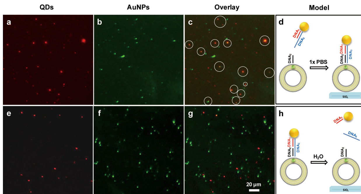
Figure 6. Membrane-encapsulated QDs functionalized with DNA-AuNP. QD-DOPC vesicles were incubated with SH-DNA and hybridized with complementary DNA-AuNP, and then imaged using PL microscopy (a, QD), darkfield scattering microscopy (b, AuNP), and then overlaid to show colocalization (c). When this sample was treated with DI water, the QD emission was no longer localized with AuNP darkfield scattering (e–g), indicating dehybridization of double-stranded DNA and disassembly of QD-DNA-AuNP structures. (d) and (h) show the models for assembly and disassembly of QD-DNA-AuNP hybrid structures.
