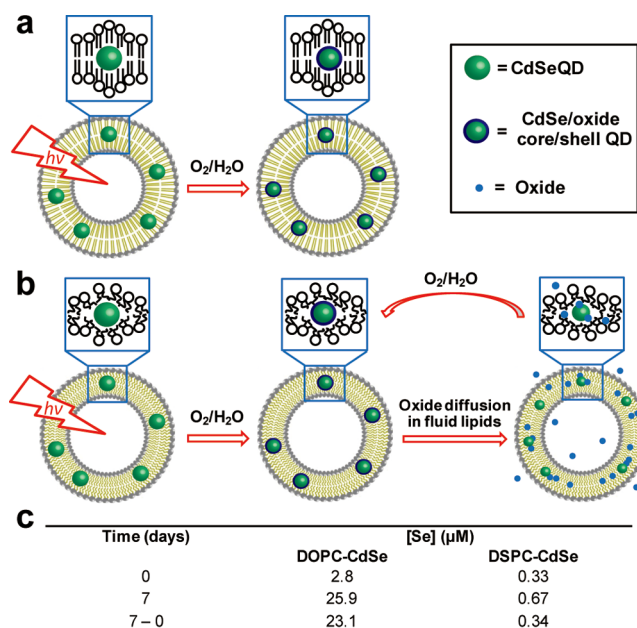
Figure 3. The mechanism of phase-dependent photo-oxidation for QDs. Proposed model of lipid phase-dependent photo-oxidation behavior for CdSe QDs in (a) gel phase lipid vesicles and (b) fluid phase lipid vesicles. Note: Surface ligands are not shown for clarity. (c) Table summarizing [Se] in the supernatant of the L-QD vesicle solutions as a function of time. Data were obtained by ICP-MS.
