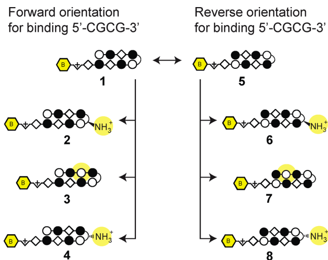
Figure 4. Panel of polyamides synthesized for assessment by Bind-n-Seq and DNA thermal stabilization for binding the 5'-CGCG-3' sequence. According to the pairing rules, polyamides 1–4 target 5'-CGCG-3' in the forward orientation and polyamides 5–8 target 5'-CGCG-3' in the reverse orientation. Structural modifications are highlighted in yellow.
