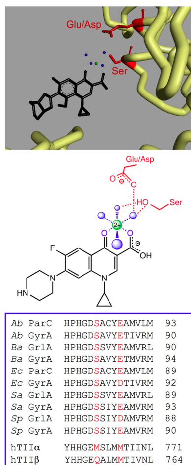
Figure 5. Quinolone-topoisomerase binding is facilitated through a water-metal ion bridge. The top panel shows the crystal structure of a moxifloxacin-stabilized A. baumannii topoisomerase IV-DNA cleavage complex. Moxifloxacin is colored black, and the noncatalytic Mg^{2+} ion that is chelated by the C3/C4 keto acid of the quinolone and participates in the bridge interaction is colored green. The four water molecules that fill out the coordination sphere of the Mg^{2+} ion are colored blue. The backbone of selected portions of the protein amino acid chain is colored yellow. The side chains of the serine and acidic residues that form hydrogen bonds with the water molecules in the water-metal ion bridge are colored red. In A. baumannii topoisomerase IV, these residues are Ser84 and Glu88, respectively. For clarity, DNA has been omitted from the picture. Protein Data Bank accession 2XKK was visualized using Discovery Studio 3.5 Visualizer (Accelrys Software Inc.). Adapted from ref 11. The middle panel shows a simplified diagram of the water-metal ion bridge. Only interactions with the protein (and not DNA) are shown. Ciprofloxacin (a representative quinolone) is colored black, and the noncatalytic Mg^{2+} , water molecules, and coordinating serine and acidic residues are colored as described above. Blue dashed lines indicate the octahedral coordination sphere of the divalent metal ion interacting with four water molecules and the C3/C4 keto acid of the quinolone. The red dashed lines represent hydrogen bonds between the serine side chain hydroxyl group or the acidic residue side chain carboxyl group and the water molecules. Adapted from ref 13. The bottom panel shows a sequence alignment of the A subunits highlighting the conserved serine and acidic residues (red) that coordinate the water-metal ion bridge. Sequences of A. baumannii (Ab), Bacillus anthracis (Ba), E. coli (Ec), Staphylococcus aureus (Sa), and S. pneumoniae (Sp) gyrase (GyrA) and topoisomerase IV (ParC/GrlA) are shown. The homologous regions of human topoisomerase IIα (hTIIα) and IIβ (hTIIβ), which lack the residues necessary to coordinate the water-metal ion bridge interaction, are shown for comparison.
