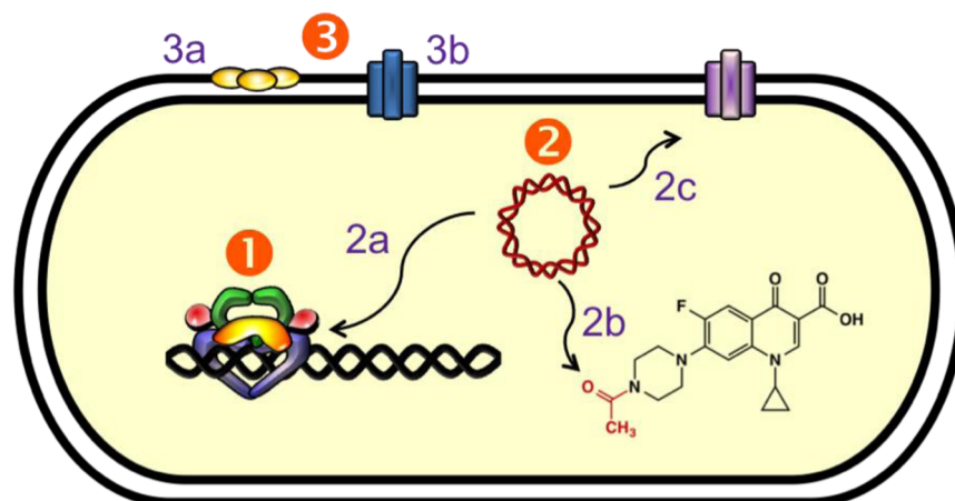
Figure 6. Mechanisms of quinolone resistance. (1) Target-mediated resistance. Mutations in gyrase and topoisomerase IV weaken quinolone–enzyme interactions. (2) Plasmid-mediated resistance. (2a) Qnr proteins (yellow) decrease topoisomerase–DNA binding and protect enzyme–DNA complexes from quinolones. (2b) Aac(6′)-Ib-cr is an aminoglycoside acetyltransferase that acetylates the free nitrogen on the C7 ring of ciprofloxacin and norfloxacin, decreasing their effectiveness. (2c) Plasmid-encoded efflux pumps decrease the concentration of quinolones in the cell. (3) Chromosome-mediated resistance. (3a) Underexpression of porins in Gram-negative species decreases drug uptake. (3b) Overexpression of chromosome-encoded efflux pumps decreases drug retention in the cell.
