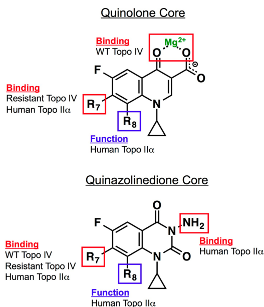
Figure 7. Roles of substituents and core elements of quinolones and quinazolinodiones that mediate drug activity against bacterial and human type II topoisomerases. Results are based on studies with B. anthracis topoisomerase IV and human topoisomerase II \alpha . 53 For quinolones, the binding of clinically relevant drugs to topoisomerase IV is mediated primarily through the water–metal ion bridge. The binding of quinolones that overcome resistance is mediated primarily by the substituent at C7. Binding of quinolones to human topoisomerase II \alpha also is mediated by the C7 substituent. The group at C8 affects the ability of quinolones to act against the human type II enzyme but is not required for drug binding. For quinazolinodiones, interactions between drugs and topoisomerase IV (wild-type and resistant) are mediated through the C7 substituent. The effects of the C7 and C8 substituents on quinazolinodione activity against topoisomerase II \alpha are the same as described for the quinolones. The N3 amino group plays a role in the binding of quinazolinodiones to the human enzyme. Adapted from ref 53.
