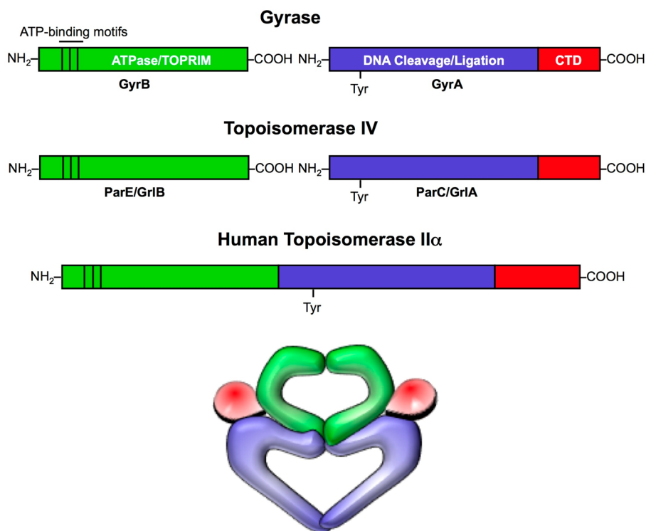
Figure 2. Domain structures of type II topoisomerases. Gyrase and topoisomerase IV are heterotetrameric enzymes consisting of two A subunits and two B subunits. The A subunits (blue and red; GyrA in gyrase and ParC and GrlA in Gram-negative and Gram-positive topoisomerase IV, respectively) contain the active site tyrosine residue that covalently attaches to the newly generated 5'-termini of DNA during the cleavage reaction. The B subunits (green; GyrB in gyrase and ParE and GrlB in Gram-negative and Gram-positive topoisomerase IV, respectively) contain the ATPase and TOPRIM domains, the latter of which binds the catalytic divalent metal ions essential for enzyme activity. The C-terminal domains (CTDs; red) of the A subunits are variable and allow gyrase to introduce negative supercoils into DNA. Human topoisomerase II \alpha is homologous to the bacterial type II enzymes. However, during the course of evolution, the A and B subunits fused into a single polypeptide chain. Therefore, eukaryotic type II topoisomerases function as homodimers. A representation of the three-dimensional structure of type II topoisomerases is shown at the bottom.
