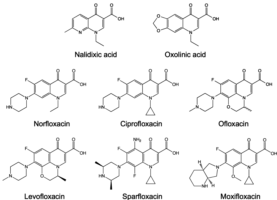
Figure 1. Quinolone structures. Nalidixic acid and oxolinic acid were the first-generation quinolones that were used most often in the clinic. Norfloxacin, ciprofloxacin, and ofloxacin are the most relevant second-generation quinolones. Levofloxacin (the levorotary isomer of ofloxacin), sparfloxacin, and moxifloxacin are newer-generation quinolones.
