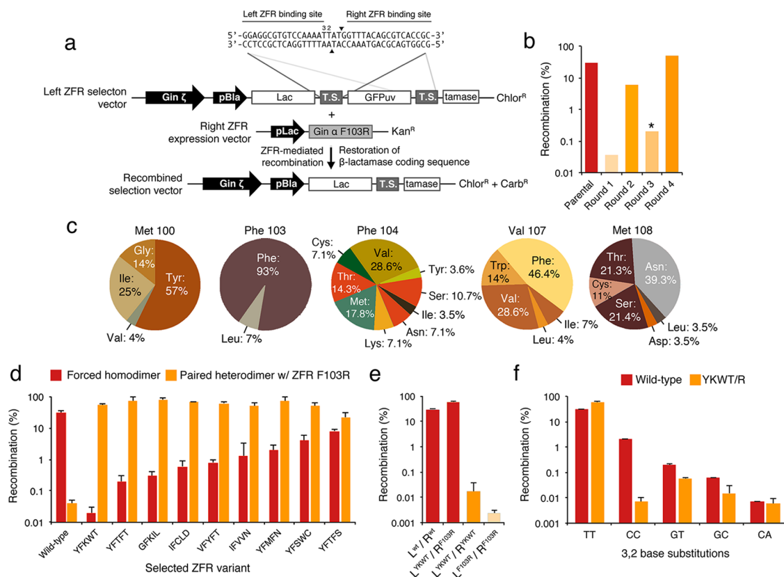
Figure 2. Re-engineering the Gin recombinase dimer interface (a) Schematic representation of the split gene reassembly system used to evaluate heterodimer-mediated recombination. Expression of active recombinase variants leads to restoration of the \beta -lactamase coding sequence and host cell resistance to carbenicillin, an ampicillin analogue. Black triangles indicate cleavage site within the DNA target. TS indicates target site. Base positions 3 and 2 of the “left” half-site are indicated. (b) Selection of Gin ζ mutants that recombine DNA when paired with Gin α F103R. Asterisk indicates the selection step in which incubation time was decreased from 16 to 4 h. (c) Mutation frequencies (%) at positions targeted for randomization in the Gin ζ catalytic domain. Twenty-eight variants were sequenced after four rounds of selection. (d) Recombination by selected Gin ζ mutants on a symmetrical DNA target upon forced homodimerization (red) or on an asymmetrical target when paired with Gin α F103R (orange). Residues selected at each dimer position are indicated including the native Phe 103. (e) Recombination by various pairs of ZFRs that contain the YKWT/R dimer interface, with wild-type control. (f) Recombination specificity of the YKWT/R dimer interface compared to wild-type. DNA targets contained substitutions at base positions 3 and 2. Error bars indicate standard deviation ( n = 3 ).
