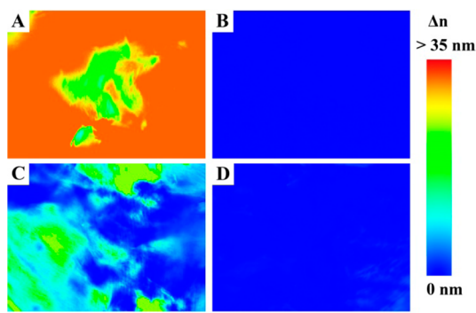
Figure 3. Polarized optical microscopy retardance images (scale bar = 100 \mu\text{m} ) of (A) Gel 1b , (B) Gel 2b , (C) Gel 1b ' , (D) Gel 2b ' . The images are taken with a sample thickness of 235 \mu\text{m} and concentration of 0.8 wt %.
