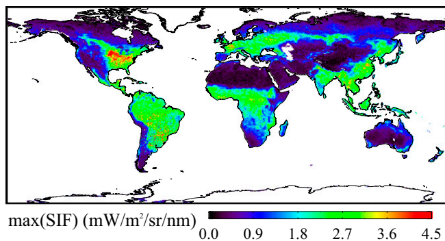
Fig. 1. Global map of maximum monthly sun-induced chlorophyll fluorescence (SIF) per 0.5^\circ grid box for 2009. SIF retrievals are performed in a spectral window centered at 740 nm (see Materials and Methods and SI Appendix, SIF Retrievals ). This map illustrates the outstanding SIF signal detected at the US CB, which shows the highest SIF return of all terrestrial ecosystems. The maximum SIF over the largest part of the US CB region is detected in July.
