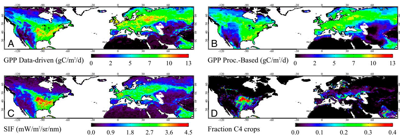
Fig. 2. Spatial patterns of maximum monthly gross primary production (GPP) per 0.5^\circ grid box for 2009 from data-driven (A) and process-based (B) models together with maximum monthly SIF at 740 nm (C). The fraction of C4 crop area (mostly corn in this region) depicts the approximate area of the US Corn Belt (D). The data-driven GPP data correspond to the MPI-BGC model (27), the process-based GPP corresponds to the median of an ensemble of 10 global dynamic vegetation models from the Trendy (“Trends in net land-atmosphere carbon exchange over the period 1980–2010”) project (28, 29), and SIF was retrieved from GOME-2 satellite measurements (26). The fraction of C4 crop data are described in Ramankutty et al. (6).
