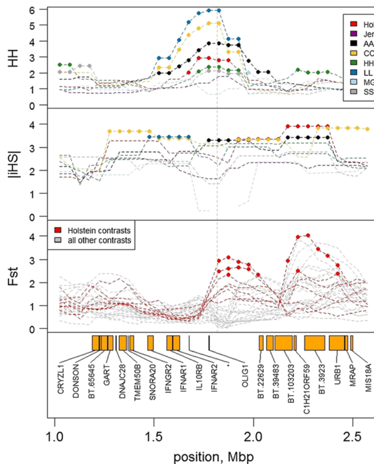
Figure 1 Haplotype homozygosity (HAPH), the integrated haplotype score ( |iHS| ) and F_{ST} near the POLLED locus. Breeds are Holstein (Hol, red), Jersey (Jer, purple), Angus (AA, black), Charolais (CC, yellow), Hereford (HH, green), Limousin (LL, blue), Murray Grey (MG, light blue) and Shorthorn (SS, grey). Points indicate windows with extreme (top 5%) values for HAPH, |iHS| or F_{ST} . F_{ST} of each breed with Holstein are highlighted in red (bottom panel). Trait units are multiples of an average window (HH, FST) or absolute standard deviations from the mean ( |iHS| ).
