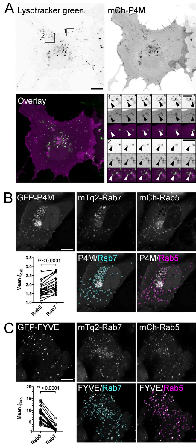
Figure 5. P4M binds endosomes/lysosomes. (A) COS-7 cells expressing mCherry (mCh)-tagged P4M were loaded with 100 nM LysoTracker green. The insets 1 and 2 are shown as a montage of images acquired at 3.9-s intervals showing motile, P4M, and LysoTracker-positive structures highlighted by the arrowheads. (B) COS-7 cells transfected with GFP-P4M, the late endosomal marker Rab7 (tagged with mTurquoise2 [mTq2]), and the early endosomal marker Rab5 (tagged with mCherry). A binary mask derived from the Rab7 and Rab5 images was used to calculate the relative intensity of the P4M signal associated with each compartment. The results from 24 cells are shown as a paired scatter plot. (C) As in B, except cells were transfected with the GFP-tagged FYVE domain from EEA1 as a marker of PtdIns3P. Bars: (main images) 10 \mu m; (insets) 5 \mu m. Statistics report the p-value from a paired Student's t test (see Materials and methods).
