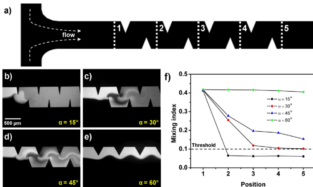
Fig. 4. Characterization of the mixing performance with different tip angles of sharp-edges. (a) Schematic of the microchannel with sidewall sharp-edges. The mixing index was characterized at five different positions (positions 1–5, indicated by the dashed white lines in the figure). (b) 15^\circ : Excellent mixing was quickly achieved after position 2. (c) 30^\circ : Acceptable mixing was achieved after position 4. (d) 45^\circ : Incomplete mixing. (e) 60^\circ : A laminar flow pattern was observed even if the piezoelectric transducer was ON. (f) Plots of mixing indices at different positions along the microchannel with different tip angles of sharp-edges.
