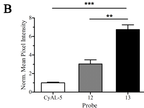
Figure 6. Ex vivo fluorescence images of excised rat prostate tumors from animals sacrificed 24 h after intravenous dosing (3.0 mg/kg) with deep-red CyAL-5 dye, probe 12, or probe 13 (A). Mean pixel intensities for the tumors normalized to the value for CyAL-5 (B). Error bars are standard error of the mean. N = 4 , ^{**}P \leq 0.01 , ^{***}P \leq 0.001 . Length scale bar = 1 cm.
