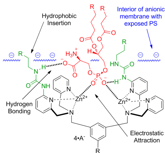
Scheme 1. Illustration of the Putative Primary and Secondary Non-Covalent Interactions between a Phosphatidylserine Head Group (Red) Embedded in an Anionic Membrane Surface (Blue) and a Zn-BDPA Core Structure (Black) with Appended 2-Amido Substituents (Green)
