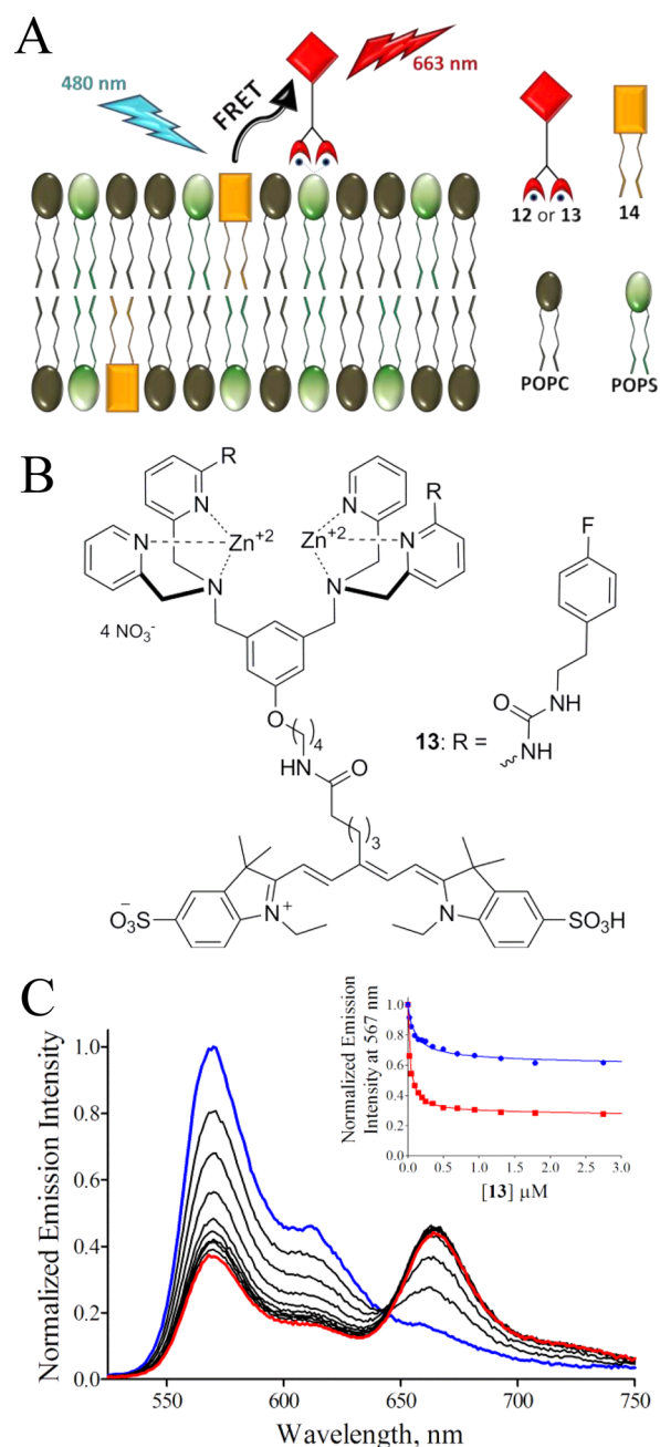
Figure 3. Schematic cartoon of the FRET titration assay (A). Chemical structure of 13 (B). FRET profiles for titration of PS-rich vesicles (10 \mu M total lipid; POPS:POPC:14, 50:49:1) and 13 (C). FRET titration curves for either PS-rich (10 \mu L total lipid; POPS:POPC:14, 50:49:1; red squares) or PC vesicles (10 \mu L total lipid; POPC:14, 99:1; blue circles) and 13 (C-inset).
