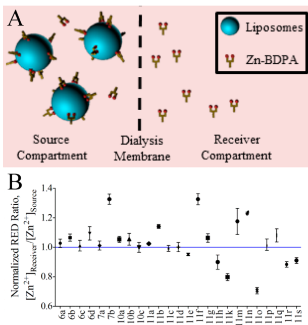
Figure 1. Schematic cartoon of the high throughput RED assay (A). RED screening results for the 25 member library of modified Zn-DPA compounds relative to the original unmodified compound, 11c (B). A low [Zn^{2+}]_{Receiver}/[Zn^{2+}]_{Source} ratio indicates compounds that have relatively high affinity for PS-rich vesicles.
