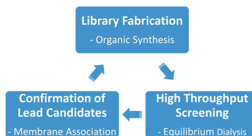
Chart 1. Library Generation and Screening
