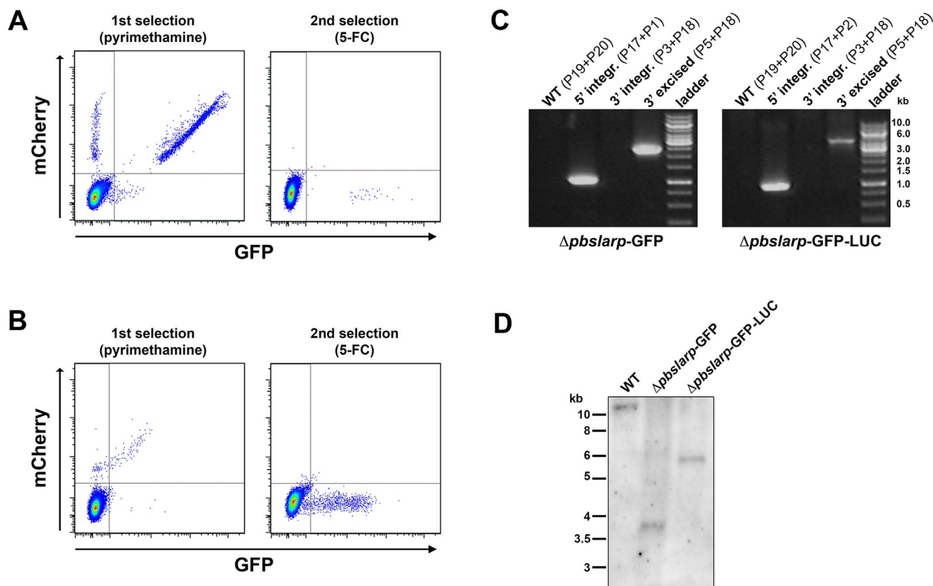
Figure 3 | Generation of drug-selectable marker-free \Delta slarp -GFP and \Delta slarp -GFP-LUC P. berghei ANKA parasites. (A–B). FACS scatter plots of parasites transfected with GOMO-GFP (A) and GOMO-GFP-LUC (B) constructs targeting PbSLARP (PBANKA_090210). The GFP + mCherry + parasite population obtained after positive selection with pyrimethamine (left panels) was replaced by a GFP + mCherry - population after negative selection with 5-FC (right panels). (C). PCR analysis of genomic DNA isolated from P. berghei WT, \Delta slarp -GFP (left panel) and \Delta slarp -GFP-LUC (right panel) parasites recovered after GOMO selection. Confirmation of the predicted recombination events was achieved with primer combinations specific for 5' integration (5' integr.) or 3' integration followed by marker excision (3' excised). Primers used for genotyping are indicated in Fig. S6 and Table S1. The absence of amplification with primer combinations specific for the WT locus (WT) and the non-excised integrated construct (3' integration) confirmed that the final populations contained only \Delta slarp marker-free parasites. (D). Southern blot analysis of genomic DNA isolated from P. berghei WT, \Delta slarp -GFP and \Delta slarp -GFP-LUC final parasite populations selected with the GOMO procedure, using a digoxigenin-labelled probe specific for the 3' homology sequence of PbSLARP . After digest with Sna BI and Afl III, the probe hybridizes to a 11.6 kb fragment in WT, a 4.0 kb fragment in recombined non-excised parasites, and a 3.6 or 5.8 kb fragment after marker excision in the final \Delta slarp -GFP and \Delta slarp -GFP-LUC parasite populations, respectively. The position of the probe and the restriction fragments are indicated in Fig. S6.
