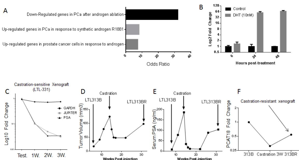
Figure 3: A, Transcripts positively associated with PCAT18 (SAM analysis, Q < 0.5\% ) were analyzed in OncoPrint for “literature defined concepts” ( p < E-4 , odds ratio > 2 ). Here we show the top 3 concepts associated with JES. B, PCAT18 expression levels in untreated LNCaP cells (Control) and cells supplemented with dihydrotestosterone (DHT, 10nM, 6-24-48h). LNCaP cells were grown in phenol red-free medium (RPMI-1640) supplemented with 10% charcoal-stripped FBS. Columns represent mean value (2 independent experiments performed in triplicate), bars standard deviation. C, Expression of 3 genes in xenografts from mice supplemented with Testosterone (Test.) (2.5mg/mouse, n=2) or after castration (1, 2, 3 weeks, n=3). LOC728606 (PCAT18) down-regulation is comparable to that of PSA. Data are from LTL-331 human prostate cancer xenografts (www.livingtumorlab.com) and normalized to the average HPRT1 expression level in testosterone-supplemented animals. HPRT1 expression is stable pre- and post-castration (unpublished microarray data). RNA extraction, retro-transcription and qPCR were performed as described in Fig. 1B legend. D, E, The living tumor lab (www.livingtumorlab.com) comprises a collection of patient-derived PCa tumor tissue xenografts, originated with a method described in ref. An androgen-dependent PCa line (LTL313B) has been exposed to castrate-levels of testosterone for a prolonged time, in order to generate a castration-resistant subline. The figures show LTL313B tumor volume (C) and serum PSA levels (D) before and after castration. Neoplastic cells were implanted in male NOD/SCID intact mice, supplemented with testosterone until castration. Serum PSA was measured and mice were sacrificed for tumor volume measurement at indicated time points, as described before[25]. At 12-16 weeks post-castration, a castration-resistant, AR-positive cell line was generated (LTL-313BR). F, PCAT18 expression was measured by qPCR in testosterone-supplemented LTL313B, castrated xenografts (3 weeks) and in a CRPC subline (LTL313BR, no testosterone supplementation).
