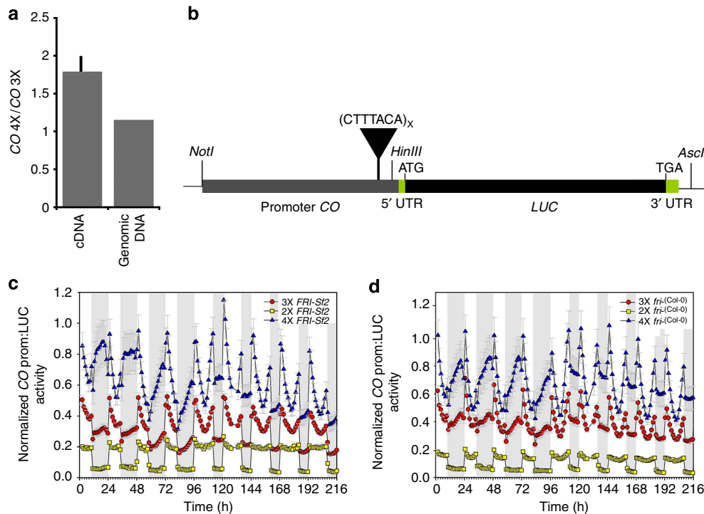
Figure 3 | CO promoter type drives differences in gene activity. (a) Expression ratio in a semi-hybrid (Col-O) heterozygote genetic background measured with pyrosequencing. Genomic DNA was used to quantify PCR biases ( n = 7 plants). (b) Luciferase gene expression in transgenic reporter lines (see Fig. 2a legend). Luciferase expression was continuously monitored in seedlings in the first 96 h under short days, followed by 120 h in long days. Experimental periods of dark are shown by the light grey boxes. Expression levels of LUC for 2X ( n = 36 plants), 3X ( n = 60 plants) and 4X ( n = 60 plants) CO promoter reporter constructs are shown for (c) FRI + and (d) fri - backgrounds. Error bars indicate s.e.m.
