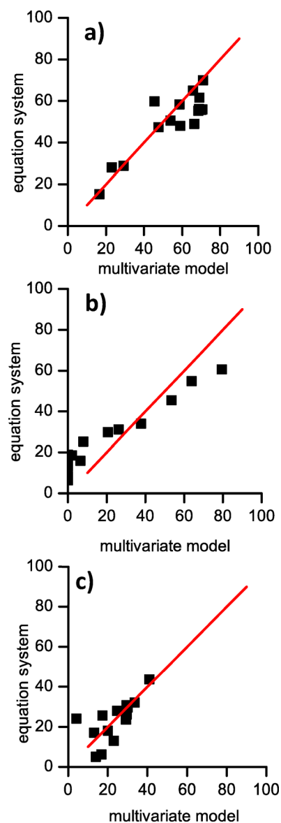
Figure 1. Plots showing the correlation between the percentages of each component calculated using equation systems and multivariate analysis of warmed samples (a) peptide, (b) lipid, and (c) polysaccharide. Please note that the red lines represent an identical percentage between the two data treatment methods and not a regression line.
