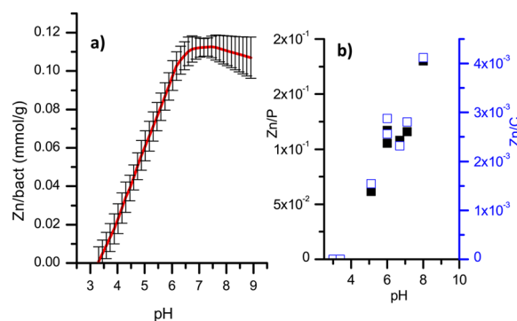
Figure 5. (a) Average adsorption of Zn(II) onto Bacillus subtilis as a function of pH (ratio between Zn(II)/dry weight biomass 0.12 mmol/g) at 24 h equilibration time. The line represents an average of four different experiments with varying amounts of bacteria. Error bars represent standard deviation. (b) Zn(II) accumulation at the surface of the sample as illustrated by the Zn/P (filled squares left y-axis) and Zn/C (empty squares right y-axis) atomic ratios. Points at low pH with a ratio of 0 represent samples where Zn could not be detected with XPS.
