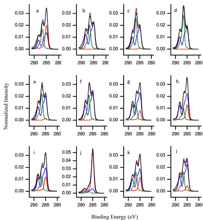
Figure 3. Fit between data and the multivariate model of the C 1s spectra: (a) pH 1.7 frozen, (b) pH 1.7 dry, (c) pH 3.4 frozen, (d) pH 3.4 dry, (e) pH 4.5 frozen, (f) pH 4.5 dry, (g) pH 6 frozen, (h) pH 6 dry, (i) pH 6 frozen, (j) pH 6 dry, (k) pH 8.2 frozen, and (l) pH 8.2 dry. The data are represented by a black line and the fit by a purple line. The components are shown in blue (peptide), red (lipid), and green (polysaccharide). All samples are Bacillus subtilis . Some differences can be seen between spectra of frozen samples and dried samples (sublimated). One sample from pH 6 displayed a dramatic change in lipid content (i, j).
