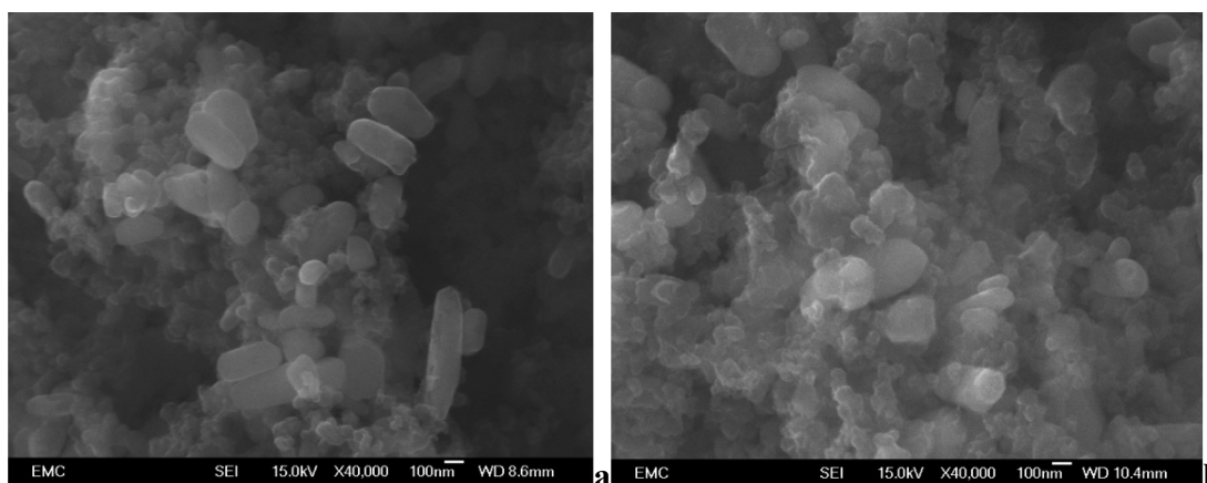
Figure 10. SEM images of electrodes containing 25% \text{LiFePO}_4 before (a) and after (b) cycling under the test regime employed in diamond. Both images have 100 nm scale bars.
