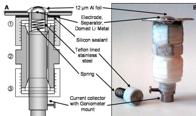
Figure 2. (a) Schematic and (b) image of the electrochemical cell used in the in situ XRD studies.
