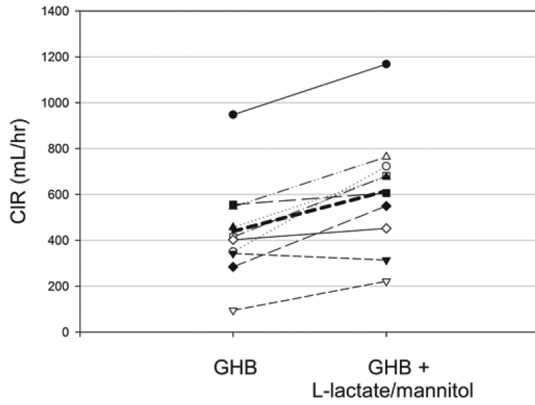
Figure 1. Individual renal clearances in 10 healthy volunteers administered GHB 50 mg/kg alone and with L-lactate/mannitol Renal clearance (CIR) of each subject is represented by individual symbols. Heavy dashed line represents mean.
