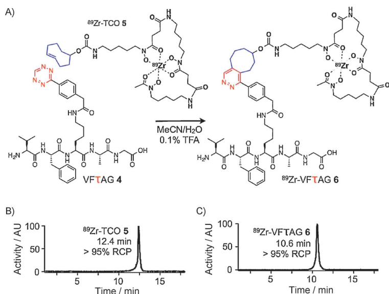
Figure 2. Chemically orthogonal synthesis of ^{89}\text{Zr} -VFTrAG (6). A) Synthesis and structure of 6, product of the chemically orthogonal reaction of VFTrAG (4) with ^{89}\text{Zr} -TCO (5); Reaction conditions: \text{CH}_3\text{CN}/\text{H}_2\text{O} (1:1, 0.1% TFA), 30 min. B) Radio-HPLC trace of 5. C) Radio-HPLC trace of 6.
