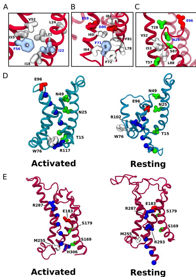
Figure 6. Coevolving residue–residue contacts. (A) Close-up of the coevolving “hydrophobic nest” that surrounds conserved hydrophobic residues F56 and I22. (B) Close-up of the coevolving “cage” that surrounds F71. (C) Coevolving network of polar and apolar residues at the extracellular mouth of the VSD. (D) Computationally modeled activated and resting states of the NavAb VSD, as described in Amaral et al. (2012). Residues of interest are labeled. (E) Computationally modeled activated and resting (C3) states of the Kv1.2 VSD, as described in Bjelkmar et al. (2009).
