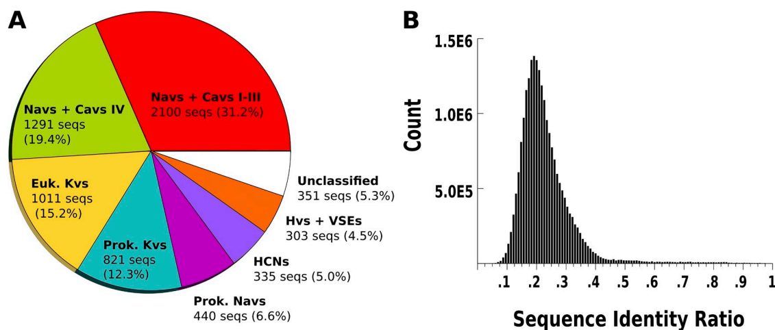
Figure 2. The sequence sample is correctly stratified and captures the VSD sequence variability. (A) Breakdown of the MSA into protein families. Navs + Cavs I-III, the first three VSDs in the pseudotetrameric voltage-gated sodium and calcium channels; Navs + Cavs IV, the fourth VSD in the pseudotetrameric voltage-gated sodium and calcium channels; Euk. Kvs, eukaryotic voltage-gated potassium channels; Prok. Kvs, prokaryotic voltage-gated potassium channels; Prok. Navs, prokaryotic voltage-gated sodium channels; HCNs, hyperpolarization-activated cyclic nucleotide-gated channels; Hvs + VSEs, voltage-gated proton channels and voltage-sensitive enzymes. (B) Histogram of pairwise sequence identities for the MSA.
