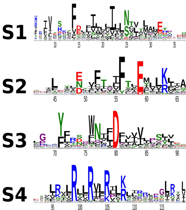
Figure 3. Sequence logos of the VSD. Black, CAVILMWF; green, TSNQY; blue, RKH; red, DE; purple, GP. Residue numbering corresponds to homologous positions in NavAb.
