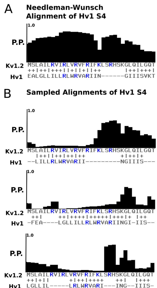
Figure 1. The register of S4 is not ambiguous. (A) Positional posterior probability of the Needleman–Wunsch optimal pairwise alignment of Kv1.2 and human Hv1. (B) Positional posterior probabilities of alignments sampled from the pair HMMs underlying the ppAlign algorithm. Each alignment represents a different possible register for the S4 helix of Hv1 with respect to Kv1.2.
