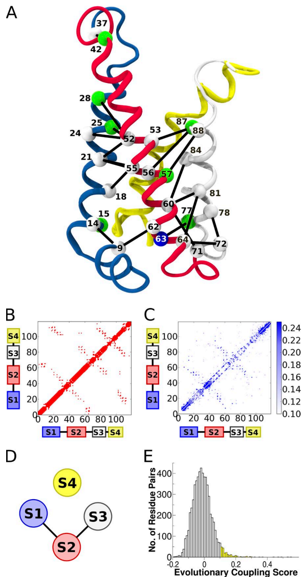
Figure 5. DCA of the VSD. (A) Cartoon representation of NavAb VSD. Top 20 evolutionarily coupled contacting nonlocal residue pairs (more than five residues apart in the primary structure). C- \alpha atoms are labeled and colored as in Fig. 3. Several top-scoring evolutionarily coupled pairs were excluded, as described in Results. Helices are colored as follows: blue, S1; red, S2; white, S3; yellow, S4. (B) Contact map for the NavAb VSD. A contact is defined between two residues if the respective C- \beta atoms (C- \alpha in the case of glycine) are within 8 Å. (C) EC map for the VSD MSA. A few couplings were much higher than the 0.25 maximum shown on the colorbar. (D) Schematic showing EC topology of VSD. (E) Histogram of the EC scores for nonlocal residue pairs. All pairs shown in C fall in the yellow region.
