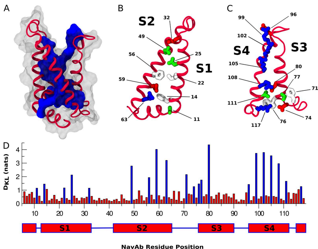
Figure 4. Single-site analysis of the VSD. (A) Cartoon representation of the NavAb VSD. Residues with a D_{KL} score greater than the 1.1-nat threshold are represented as a contiguous blue surface. Residues with a D_{KL} score below the threshold are transparent. (B and C) Helices S1–S4 of the NavAb VSD. Residues with a D_{KL} score greater than the 1.1-nat threshold are represented as licorice and colored as in Fig. 1. (D) D_{KL} score by NavAb residue position with residue positions above the 1.1- D_{KL} threshold represented as blue bars.
