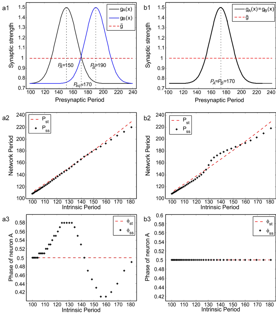
Fig. 9 Period and phase locking when both synapses follow the synaptic plasticity profile. Dashed line in all panels shows the case with two static synapses. a1 Synaptic plasticity profiles of the two synapses chosen to have different preferred periods at 150 and 190. a2 Network period as a function of the intrinsic periods. a3 Phase \phi of neuron A with respect to B as a function of intrinsic period. b1–b3 Same as a1–a3 but with identical synaptic plasticity profiles (preferred period at 170)
