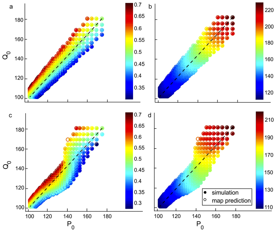
Fig. 11 Coupling of non-identical M–L neurons. The phase of neuron A ( a and c ) and the period of the network ( b and d ) for coupled neurons with different intrinsic periods are shown for static synapses ( a and b ; \bar{g} = 0.1 ) and when the network follows the synaptic plasticity profile ( c and d ; P_A = 150 , P_B = 190 ). The axes are the intrinsic periods of the two neurons. Plasticity adds nonlinearity to the period and phase distribution. Filled circles denote simulation results whereas open circles denote the map predictions. The map yields predictions very close to the simulations in most cases
