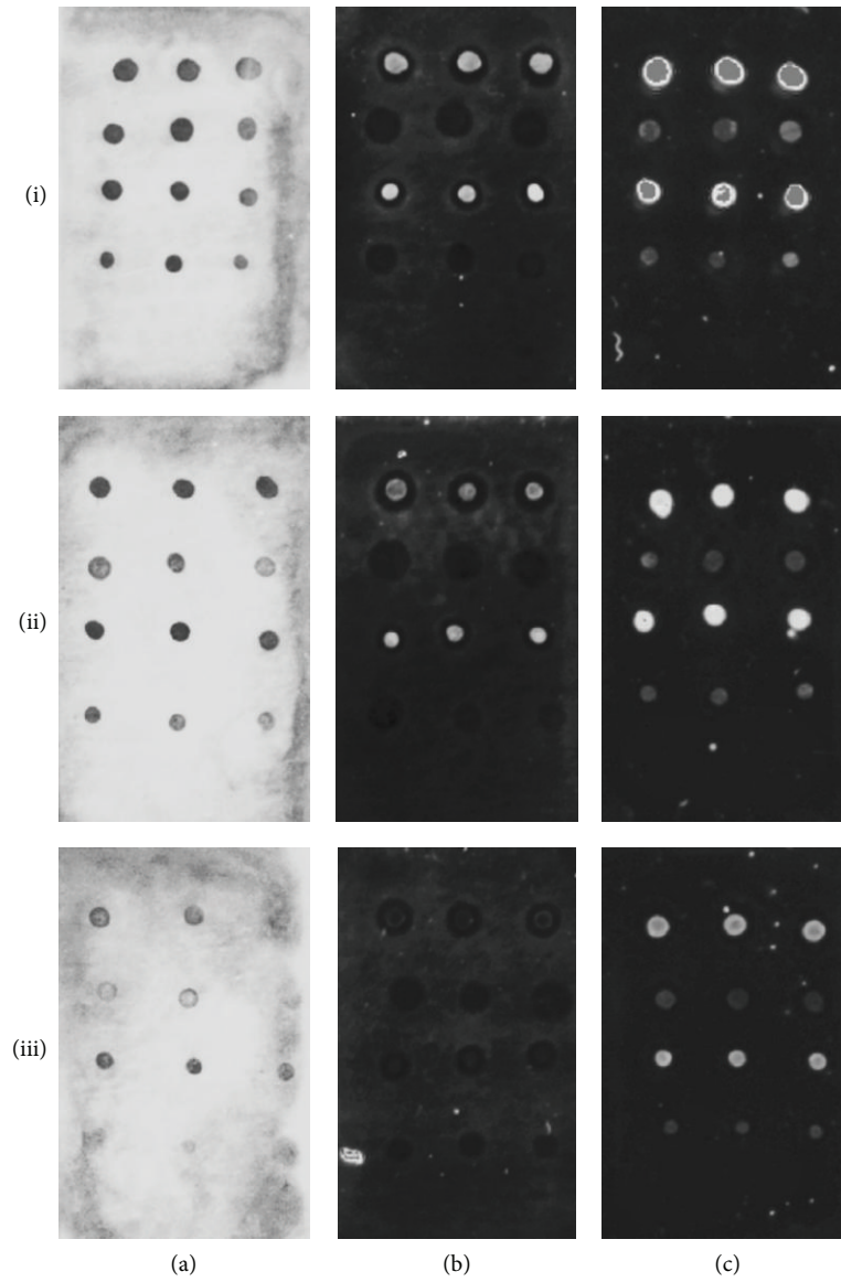
FIGURE 2: Biodyne C membrane-macroarray images obtained for optimization experiments with different labeling: (a) biotin, (b) Cy3, and (c) Cy5 and zipcode-oligonucleotides spotted at different concentrations: (i) 1 \mu\text{M} , (ii) 0.1 \mu\text{M} , and (iii) 0.01 \mu\text{M} .
