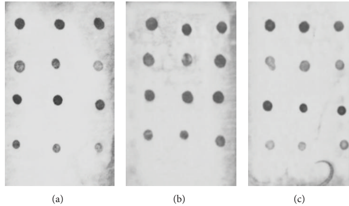
FIGURE 4: Biodyne C membrane-macroarray images obtained for optimization experiments with biotin labeling and different ligase enzymes: (a) pfu DNA ligase, (b) taq DNA ligase, and (c) ampligase.
