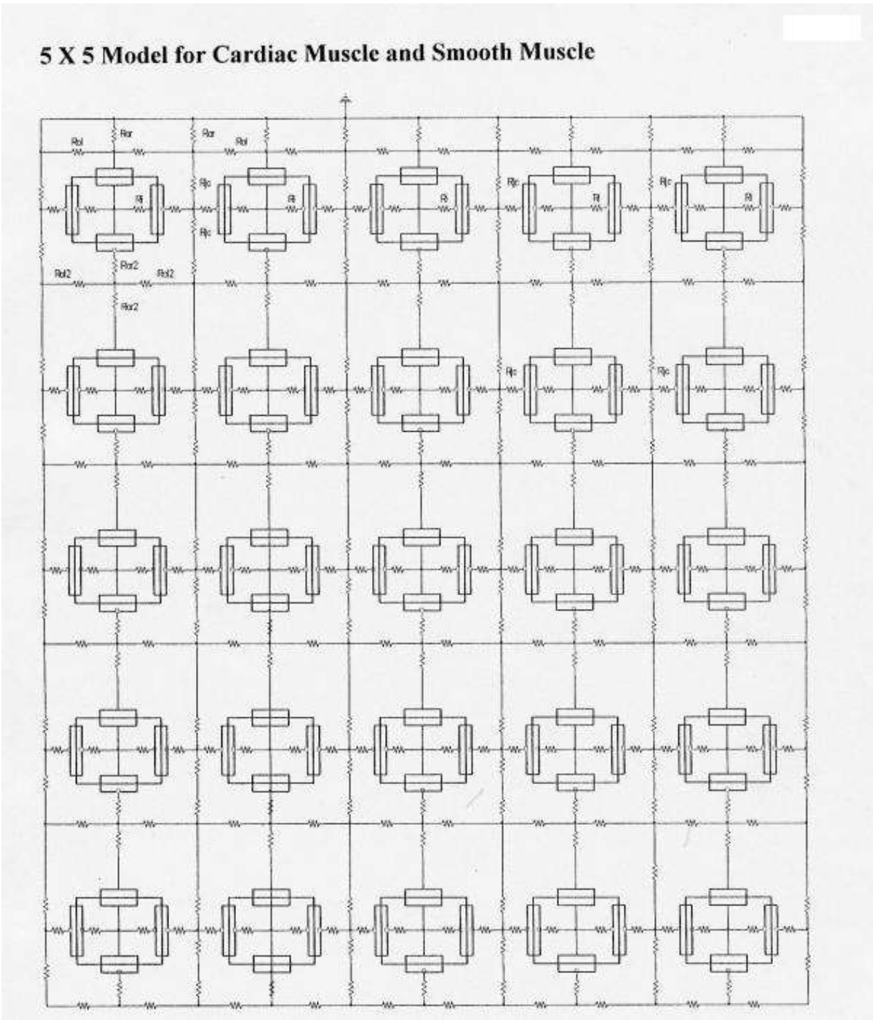
Figure 1 Diagrams of the arrangement of the myocardial cells and smooth muscle cells, basic units, and key resistances for the 5 × 5 model: 5 parallel chains (A – E) of 5 cells each (1 – 5). There were no low-resistance connections between cells within a chain or between chains. The surface membrane of each cell was represented by 2 basic units (one upwards and one inverted), and each junctional membrane by one unit each. The radial junctional cleft resistance ( R_{jc} ) is depicted, as is the longitudinal resistance of the interstitial space between the chains. Propagation of simulated action potentials was examined when only one cell of one chain was electrically stimulated (usually cell #1 of the A-chain (cell A1)).
