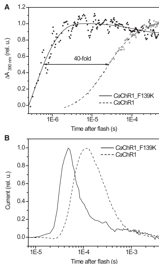
FIGURE 6 (A) Absorbance changes monitored at 390 nm in WT CaChR1 (open circles, dashed line) and its F139K mutant (solid circles, solid line) in response to a 6-ns laser flash (532 nm). The arrow shows the difference in the time of the half-maximal amplitude of the signal. (B) Outward proton transfer currents recorded upon laser excitation from WT CaChR1 (dashed line) and its F139K mutant (solid line) expressed in HEK293 cells at the reversal potential for channel currents to minimize their contribution to the signal kinetics. The current kinetics is limited by the time resolution of the measuring system. In both panels the signals were normalized to their maximal values.
