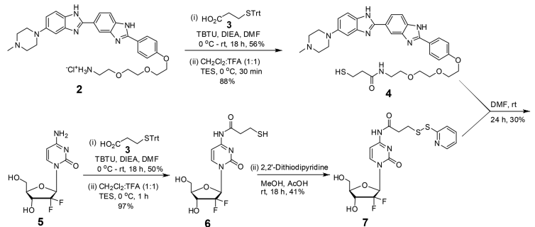
Scheme 1. Synthesis of H-gemcitabine (1)
