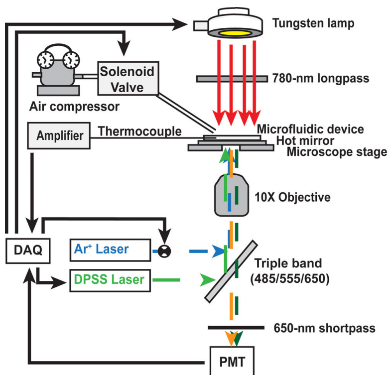
Figure 1. Schematic of instrumentation for frequency-encoded fluorescence detection during IR-qPCR
