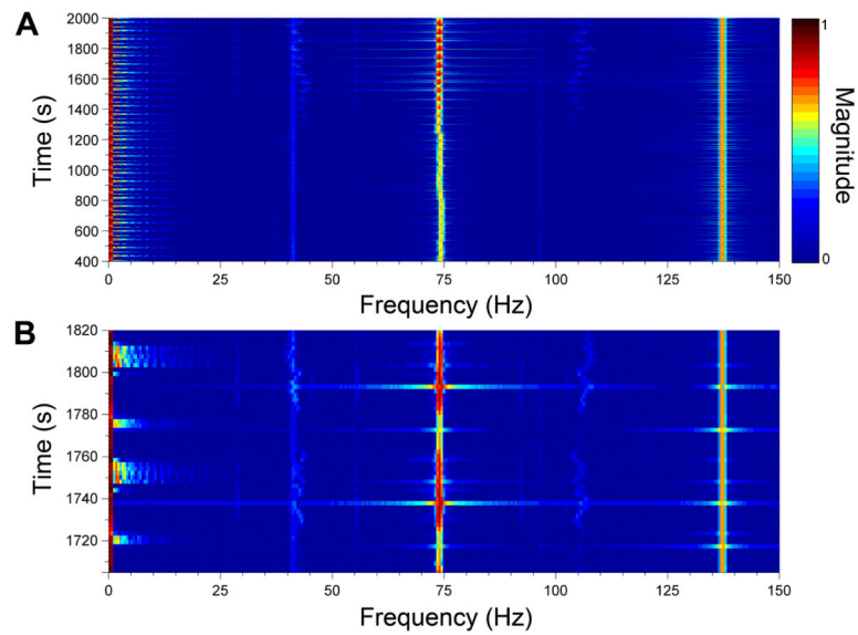
Figure 3. Spectrogram of two-color DNA amplification
