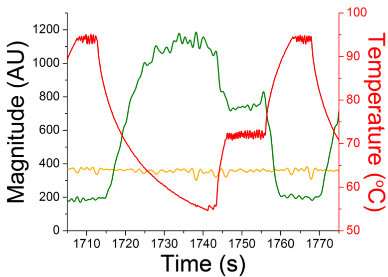
Figure 4. Extracted fluorescence signals plotted with temperature
