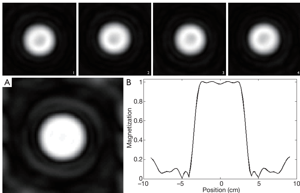
Figure 4 Excitation profiles of the 4 individual RF pulses; (A) their combined excitation profile; (B) 1D excitation profile along the central line. The excitation error of its passband based on Eq. [1] was \sim 0.2 .
