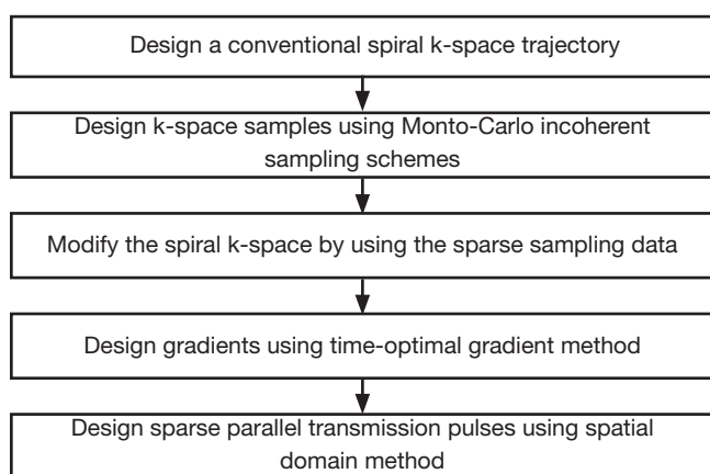
Figure 1 Design procedure of the sparse transmission pulses on randomly perturbed spiral k-space trajectory.
