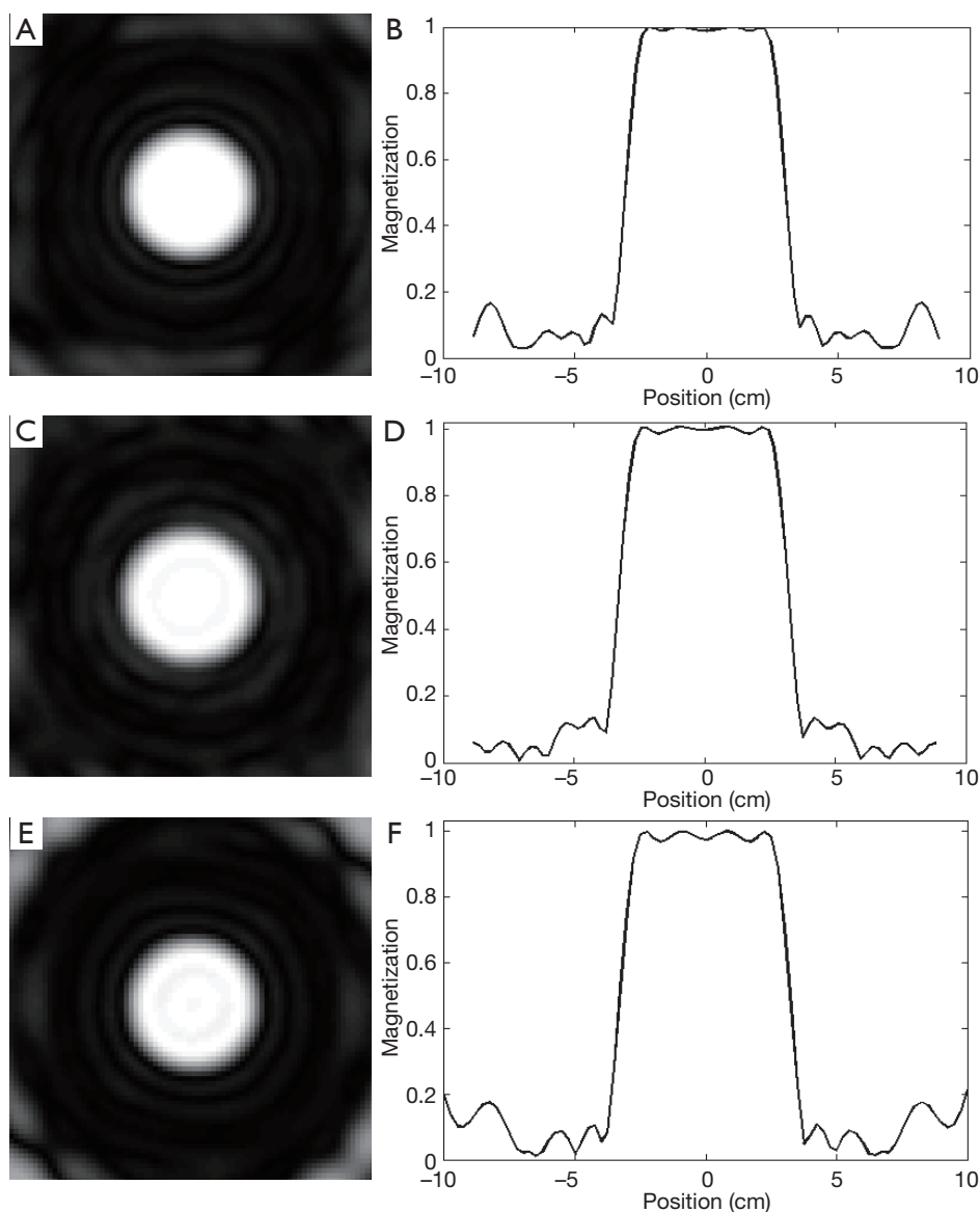
Figure 5 (A,B) 2D and 1D excitation profiles of the non-accelerated transmission (i.e., reduction rate of 1); (C,D) 2D and 1D excitation profiles of the sparse parallel transmission at the reduction rate of 2 using proposed randomly perturbed spiral trajectory; (E,F) 2D and 1D excitation profiles of an RF pulse on regular spiral k-space trajectory for comparison purpose. The passband error of the regular spiral RF pulse was in the region of 0.3, which was worse than that of the proposed method (0.2).
