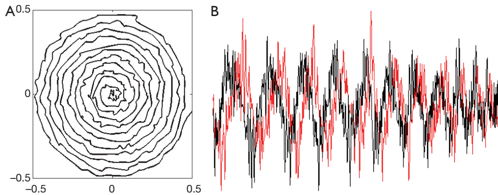
Figure 3 The randomly perturbed spiral k-space trajectory with the range from -0.5 to 0.5 on both directions (A), and (B) x (black) and y (red) gradient waveforms generated based on the proposed perturbed spiral k-space trajectory.
