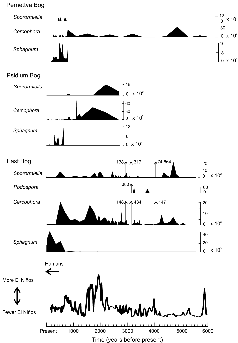
Figure 2 Variation in concentration (per \text{cm}^3 of sediment) of spores of coprophilous fungi over time at Pernettya, Psidium and East Bog. The timing of expansion of Sphagnum at each site, as well as possible drivers behind tortoise loss, is also illustrated. The first known human presence in the Galápagos archipelago occurs at AD 1535. The El Niño frequency curve for the Galápagos is modified from Conroy et al. (2008) and is based on proxy records of % sand occurrence in lake sediments from El Junco lake, San Cristóbal Island; post-AD 1850 data have been excluded as a result of likely anthropogenic impact on the record (Conroy et al. 2010).
