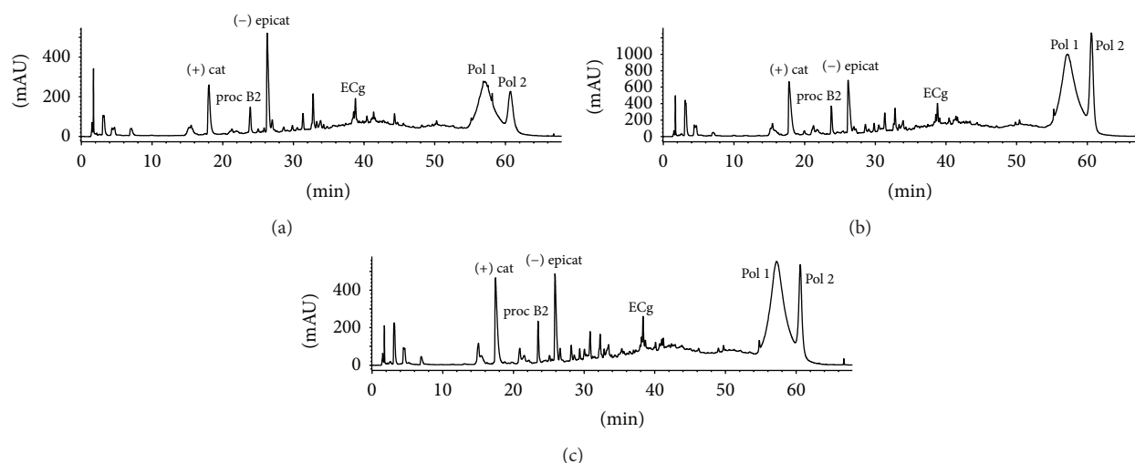
FIGURE 1: Chromatographic profiles at 280 nm of GSEs from Pinot 2011 (a), M. Palieri VIN1 2010 (b), and M. Palieri VIN1 2011 (c). (+) cat: (+)-catechin; proc B2: procyanidin B2; (-) epicat: (-)-epicatechin; ECg: epicatechin gallate; Pol 1 and Pol 2: polymeric flavan-3-ols with galloylated residues and a degree of polymerization \geq 4 , determined by mass spectrometry.
