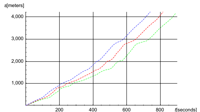
Figure 11 The accumulated simulated distance (s) in meters as functions of time (t) in seconds. Notes: Red, baseline; blue, m = 62.5 kg; green, m = 92.5 kg (where m is body mass).
