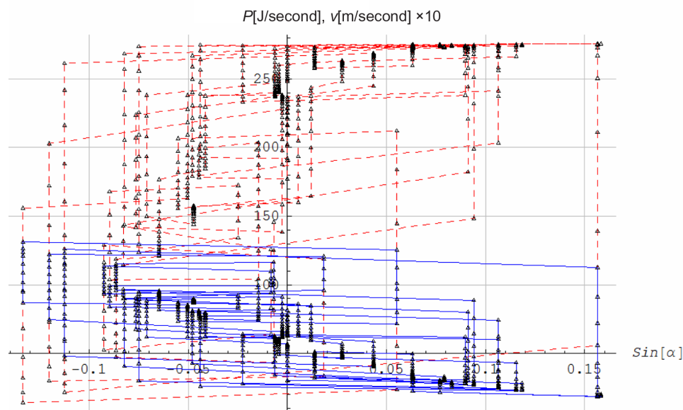
Figure 3 Blue: Locomotive power (P) versus inclination sin(α). Red: Speed (v) × 10 versus inclination sin(α).
