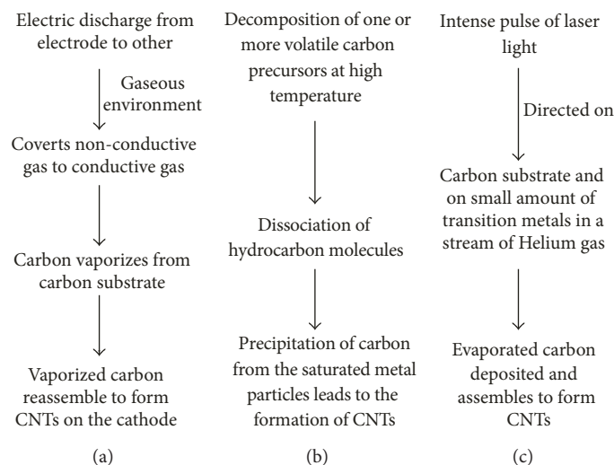
FIGURE 3: Mechanism of carbon nanotube synthesis: (a) Arc discharge method, (b) chemical vapor deposition method, and (c) laser ablation method.
