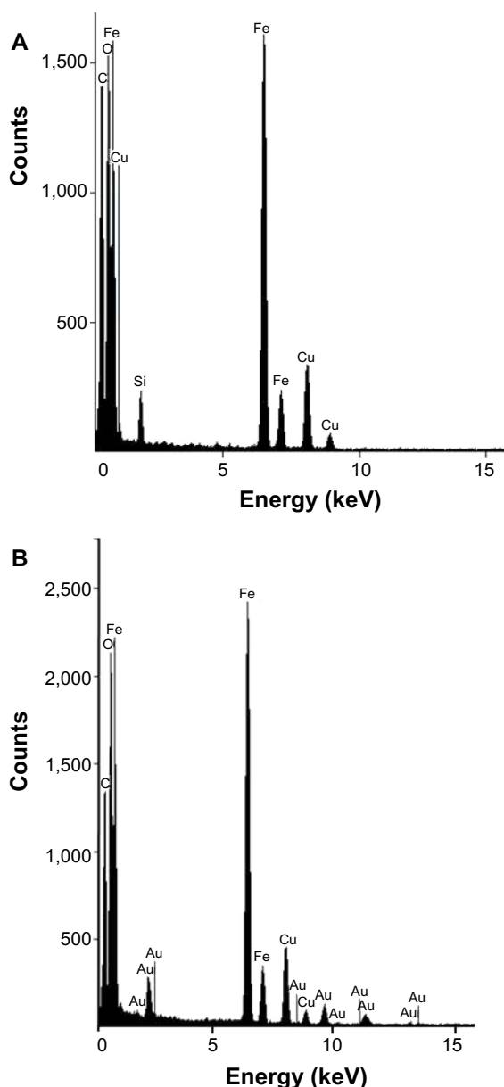
Figure 3 Energy-dispersive X-ray spectra of \text{Fe}_3\text{O}_4 nanoparticles functionalized with aminosilane ( \text{Fe}_3\text{O}_4@NH_2 ) (A) and with gold ( \text{Fe}_3\text{O}_4@Au ) (B).
