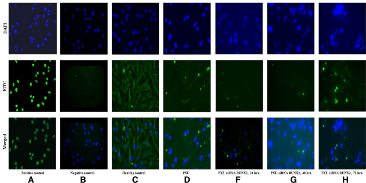
Figure 8 Analysis of apoptosis by TUNEL staining in human fibroblasts (n = 6) compared to control cells (n = 5) (×20). Counter staining was performed using DAPI nuclear staining and pictures were taken using DAPI (upper row), FITC (fluorescein isothiocyanate; middle row) and Merged (lower row) filters. Results are shown for a positive and negative control (A, B), healthy control fibroblasts (C), PXE fibroblasts (D) and PXE fibroblasts transfected with RUNX2 siRNA respectively 24 (E), 48 (F) and 72 hours (G) following transfection. PXE fibroblasts show smaller nuclei on the DAPI stain and increased TUNEL staining in the cytoplasm of fibroblasts compared to controls, reflecting a three-fold increase of apoptosis (2,08% vs 0,69% respectively, p < 0.05 ). Twenty-four and 48 hours post-transfection with RUNX2 siRNA, a decrease of apoptosis can be seen, whereas after 72 hours no difference can be observed compared to untreated PXE fibroblasts. Scale bar = 20 \mu m.
