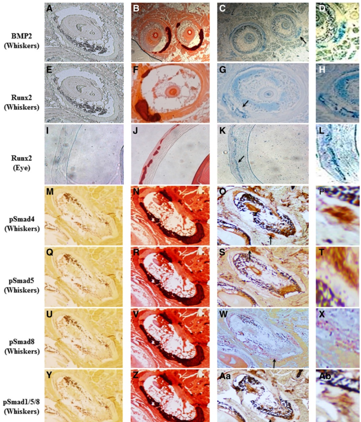
Figure 2 Staining results for the BMP2-SMADs-RUNX2 pathway in whisker and eye sections from the Abcc6 KO mouse (×10). Negative controls are shown in the first column (A, E, I, M, Q, U, Y). Alizarin Red stainings confirm profound calcification in the connective tissue capsule of the whiskers (B, F, N, R, V and Z) and Bruch's membrane of the eye (J). Immunohistochemical staining of adjacent slides with antibodies against respectively Bmp2 (C), Runx2 (G, K), pSmad4 (O), pSmad5 (S), pSmad8 (W) and pSmad1/5/8 (Aa), shows positive staining for all, co-localizing with the mineralization foci. Arrowed areas of positive staining have been magnified (×20). Scale bar = 100 μm. n = 5 each.
