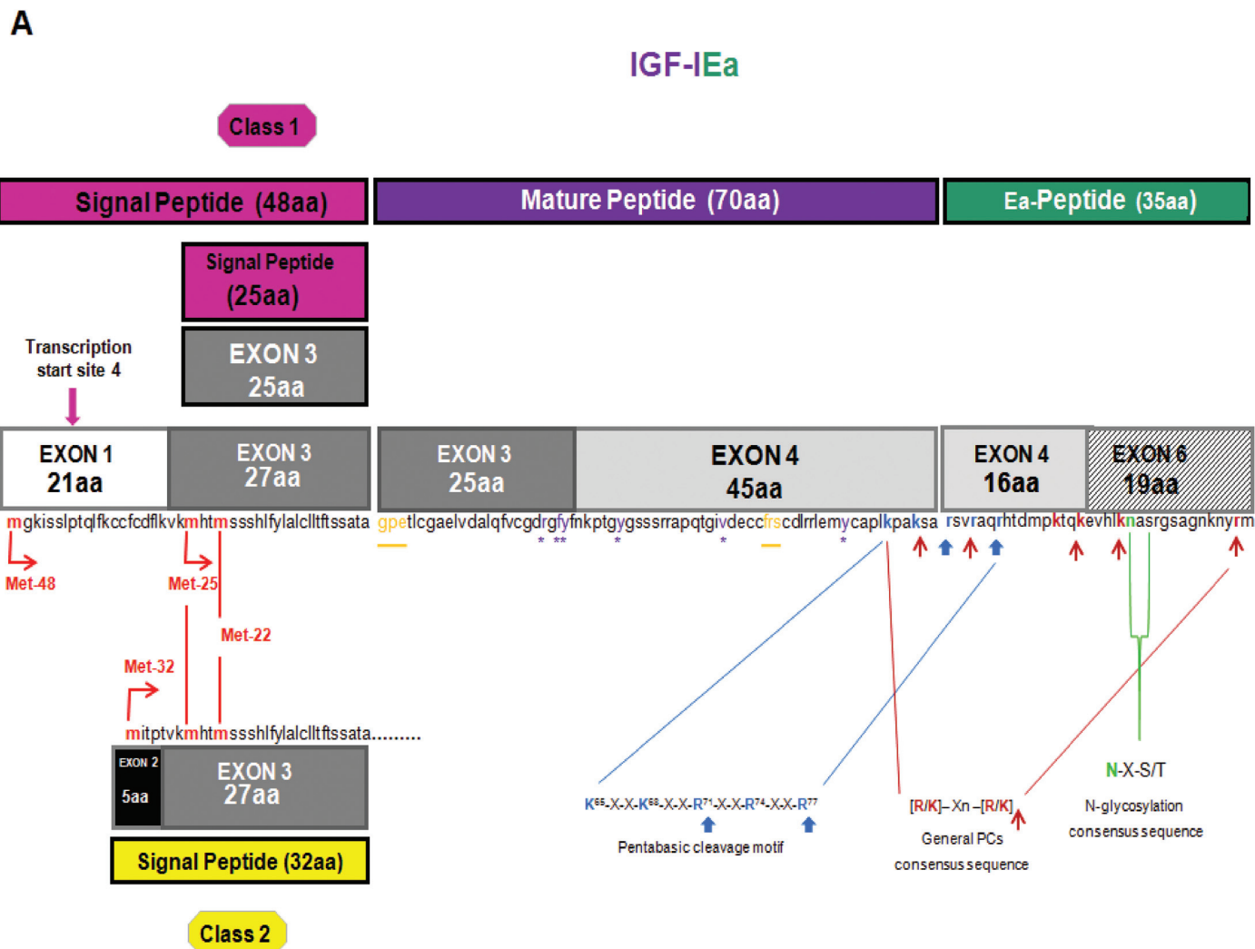
Figure 1. Gene structure, alternative splicing, amino acid sequence and posttranslational modifications of human IGF-I. Posttranslational cleavage of pro-IGF-I polypeptides can occur at a unique pentabasic motif and at sites containing the general PC consensus sequence (panels 1A–C; potential processing sites are indicated by arrows; see text for details). Only the Ea-peptide of human IGF-I contains an N-linked glycosylation site. Mature IGF-I peptide residues that interact with IGF-BPs are shown in orange color and underlined whereas residues that interact with IGF-IR are in purple color and marked with an asterisk (*) (panel 1A).
