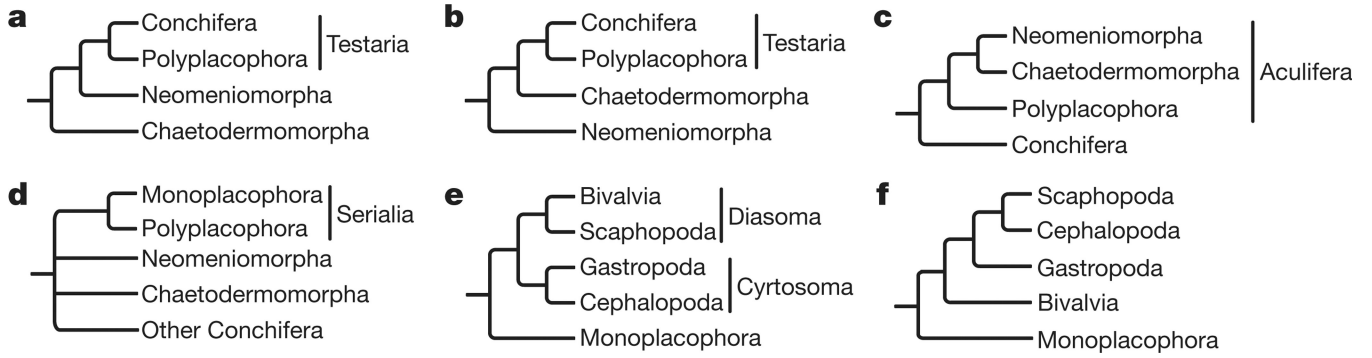
Figure 1. Leading hypotheses of molluscan phylogeny
