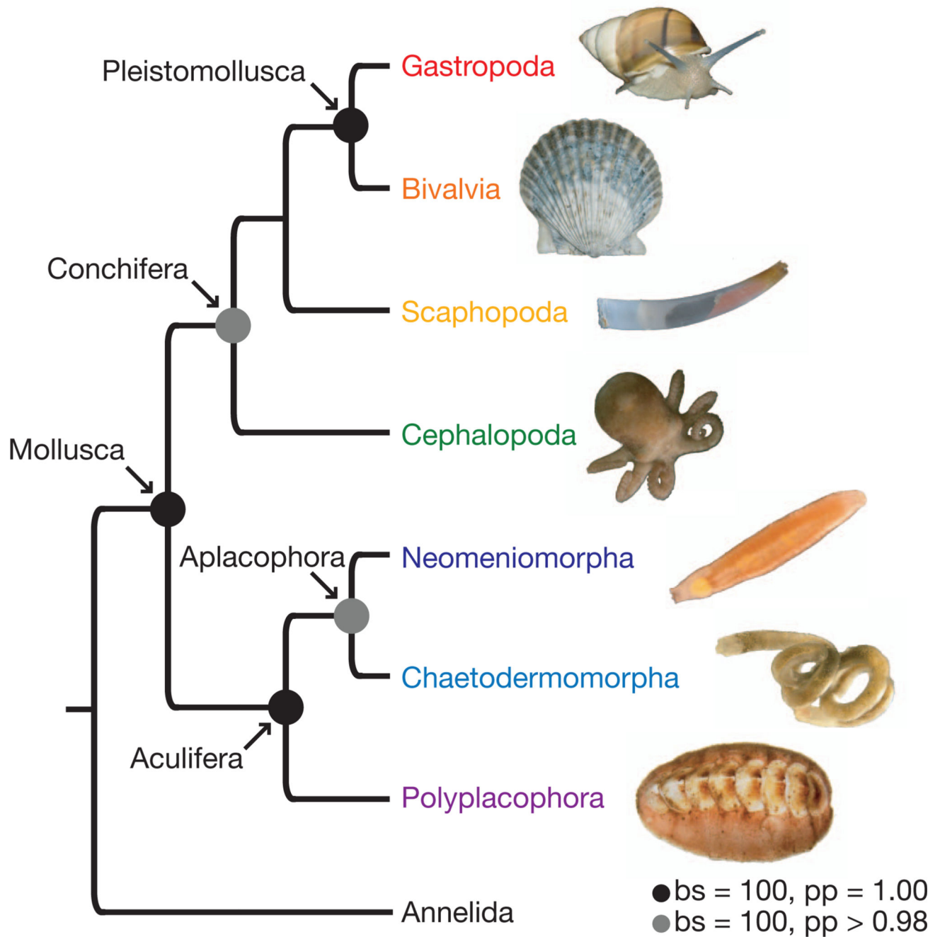
Figure 4. Deep molluscan phylogeny as inferred in the present study
