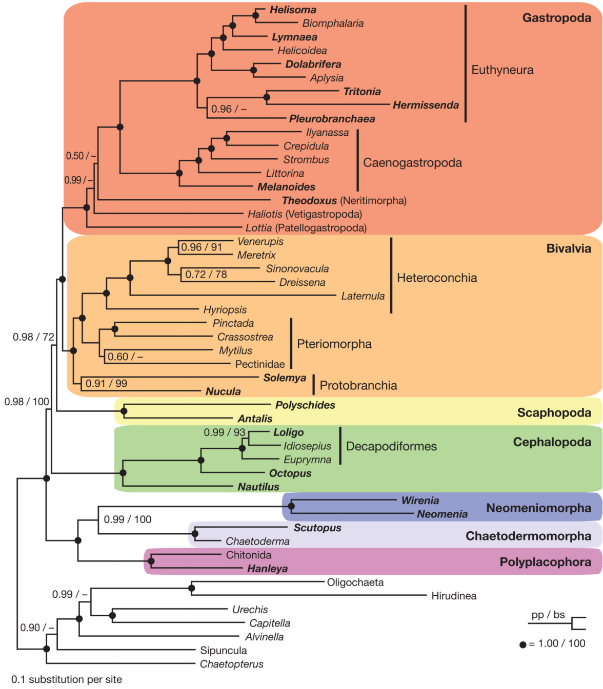
Figure 2. Relationships among major lineages of Mollusca based on 308 genes Bayesian inference topology shown with ML bootstrap support values (bs) >50 and posterior probabilities (pp) >0.50 are listed at each node. Filled circles represent nodes with bs = 100 and pp = 1.00. Taxa from which new data were collected are shown in bold.
