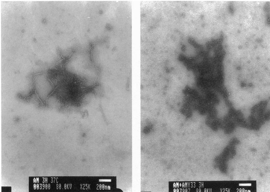
FIG. 2. Electron micrographs of \beta -amyloid aggregates in the absence (Left) or presence (Right) of mAb AMY-33. (Bars = 0.2 \mu m.)
